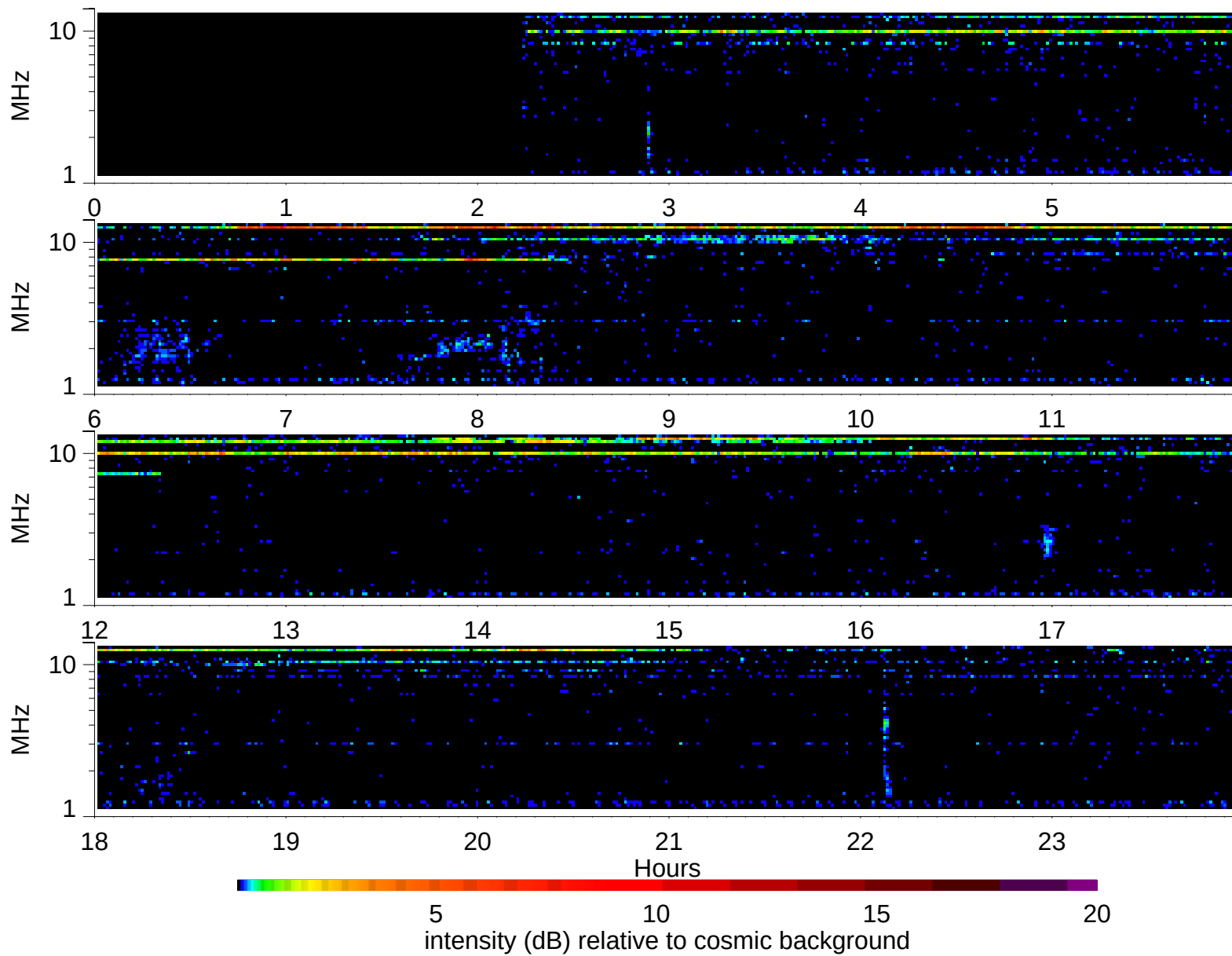
Wind Waves RAD2 receiver: 2006/5/10
