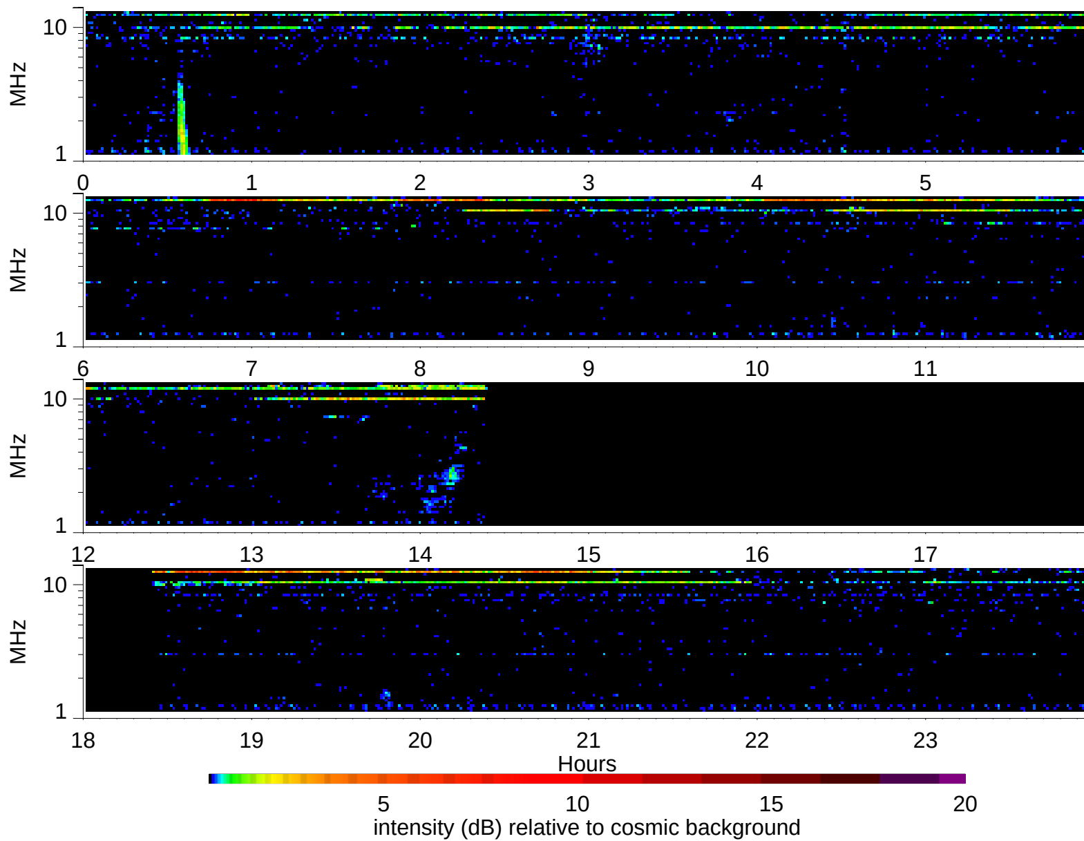
Wind Waves RAD2 receiver: 2006/5/11
