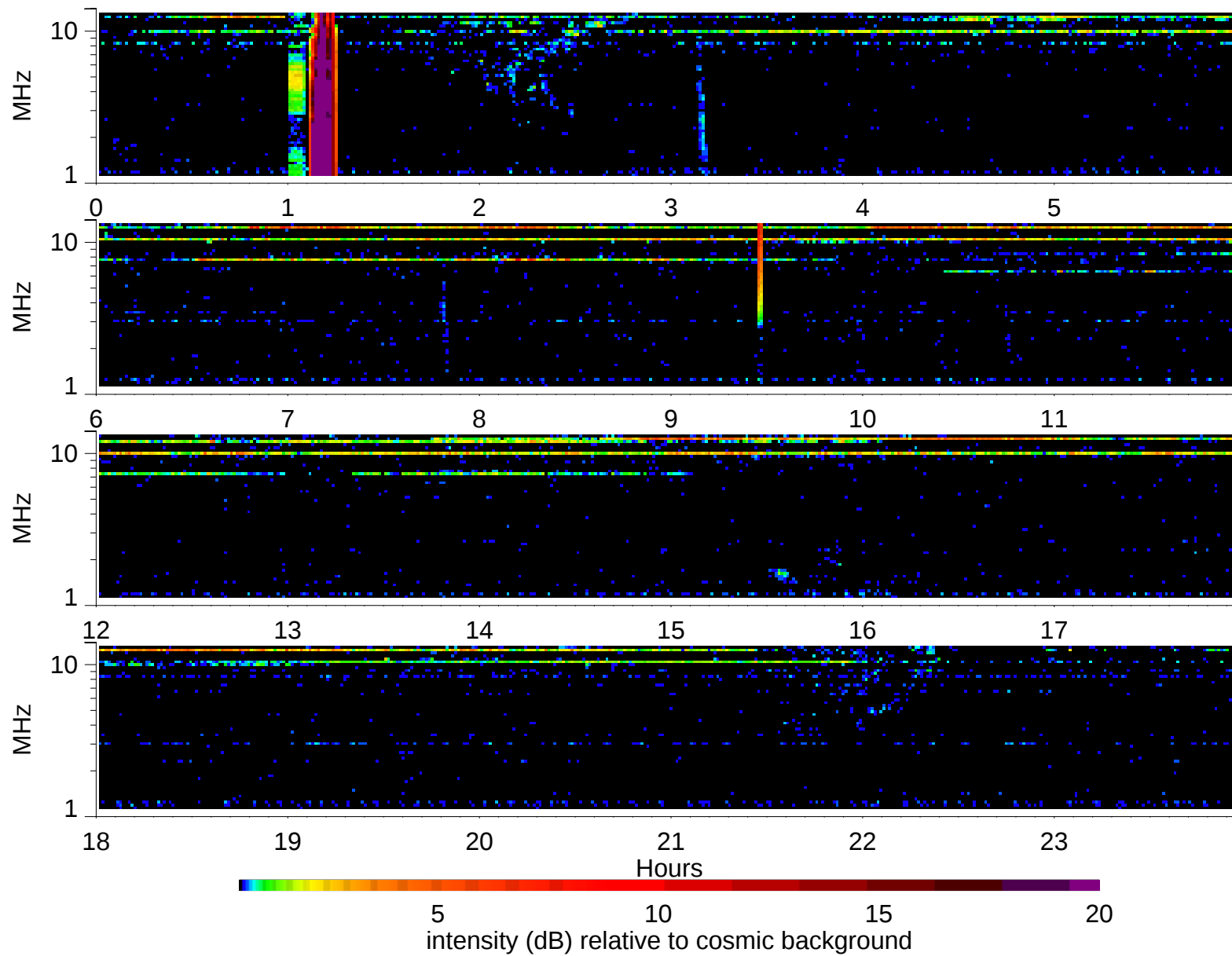
Wind Waves RAD2 receiver: 2006/5/12
