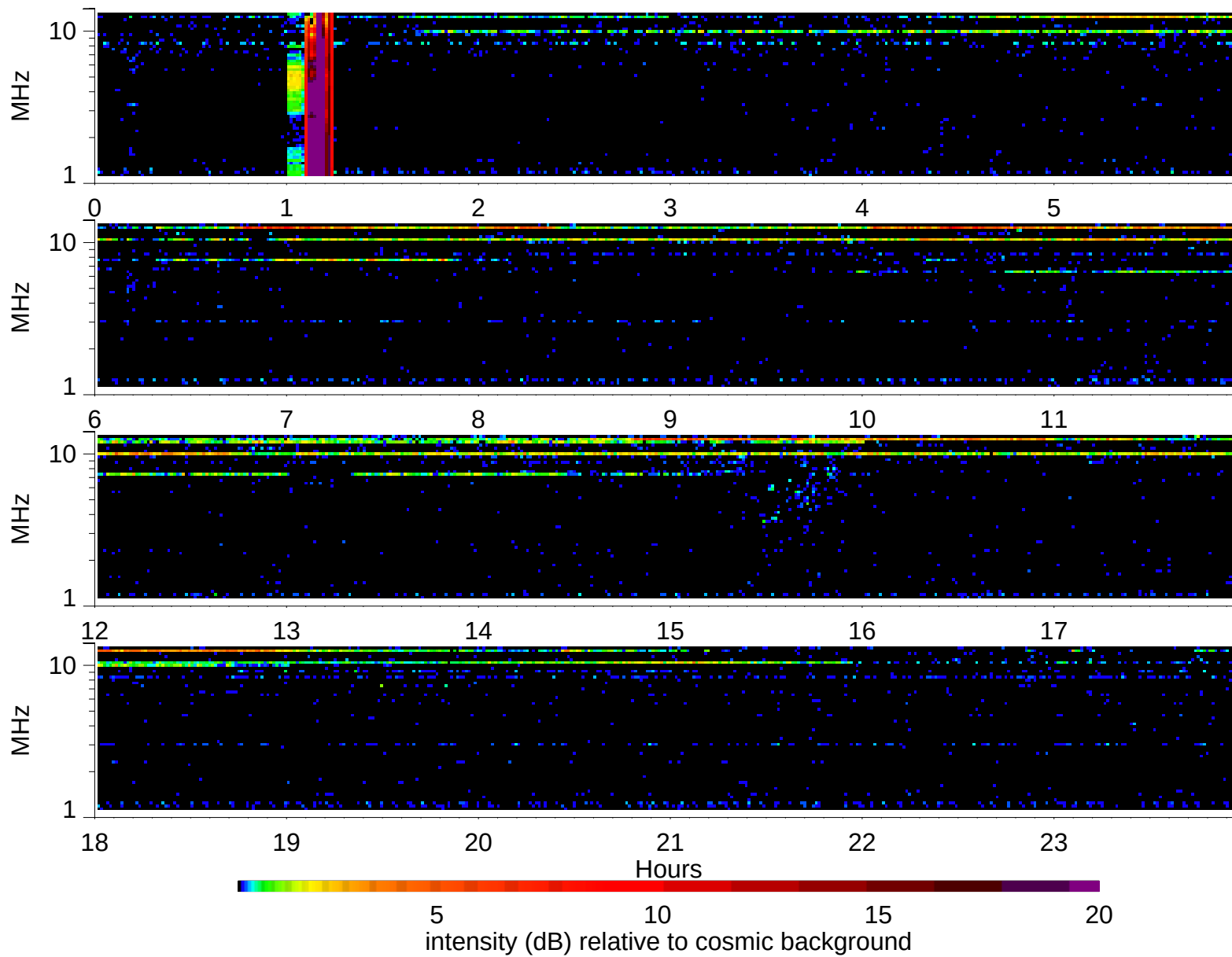
Wind Waves RAD2 receiver: 2006/5/14
