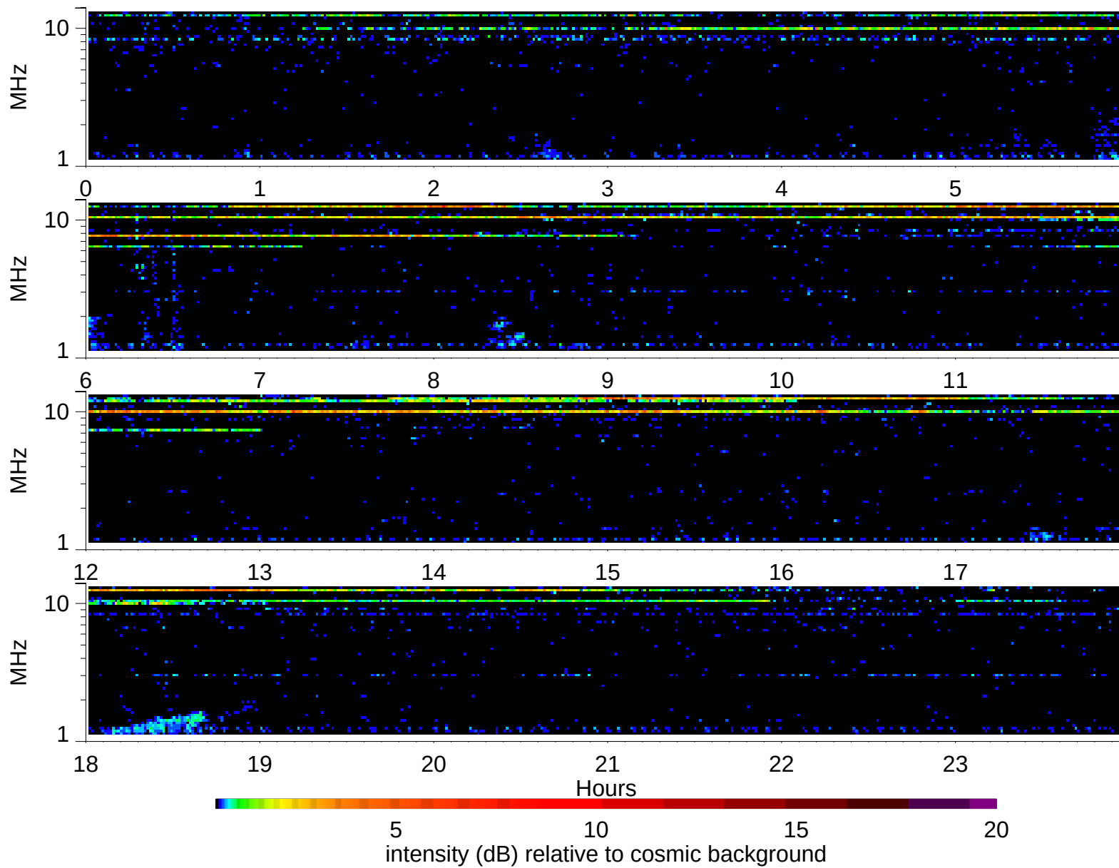
Wind Waves RAD2 receiver: 2006/5/17
