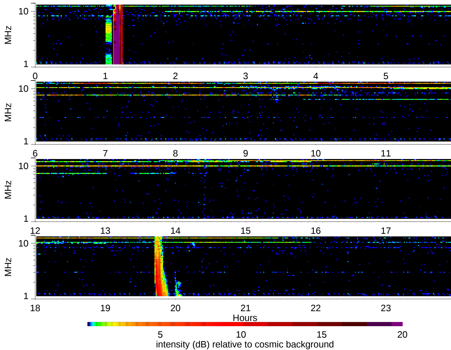
Wind Waves RAD2 receiver: 2006/5/22
