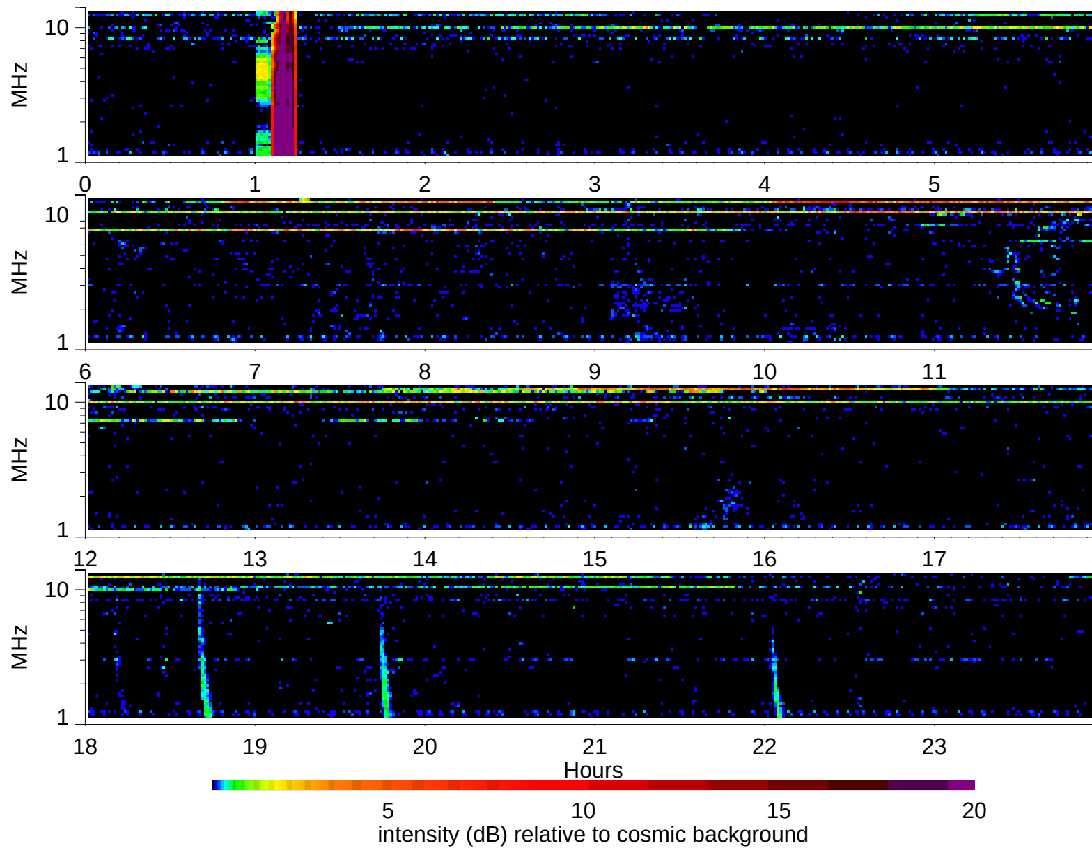
Wind Waves RAD2 receiver: 2006/5/24
