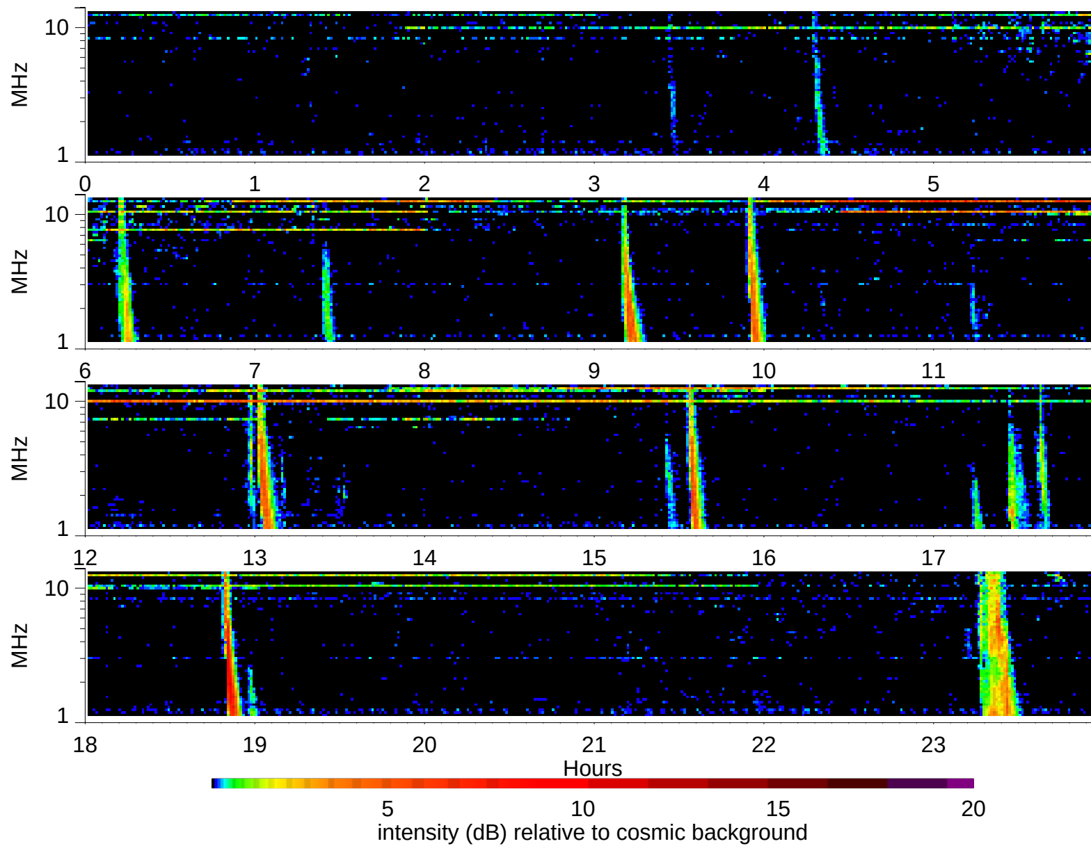
Wind Waves RAD2 receiver: 2006/5/25
