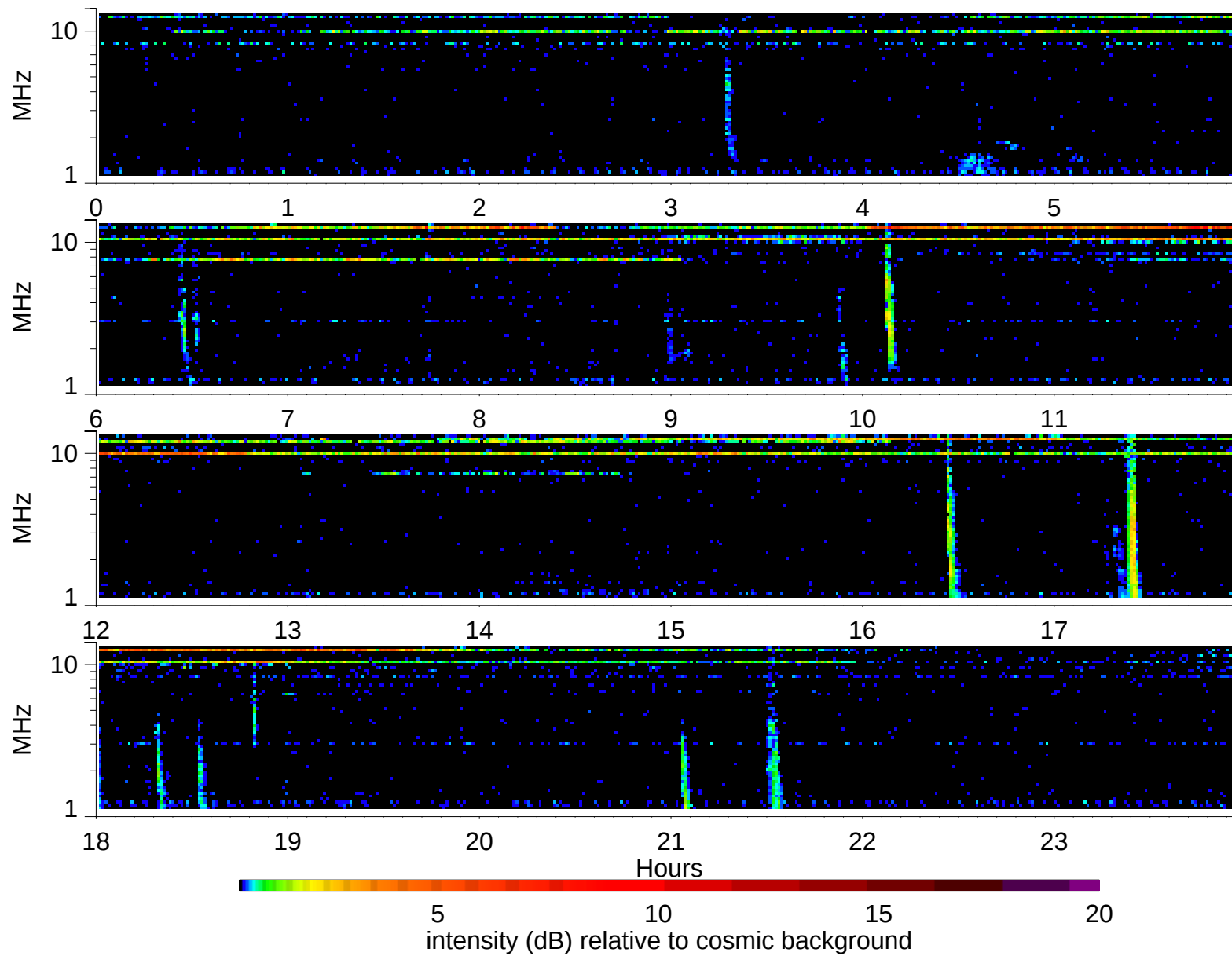
Wind Waves RAD2 receiver: 2006/5/29
