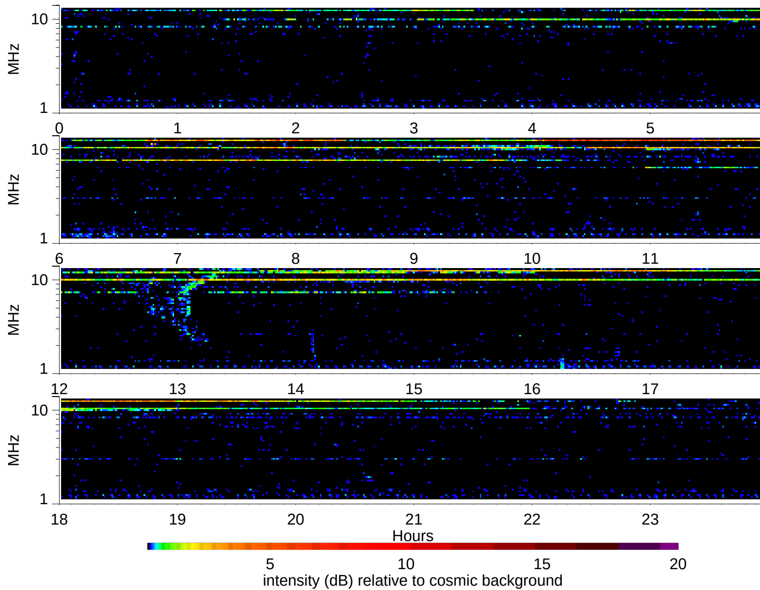
Wind Waves RAD2 receiver: 2006/5/31
