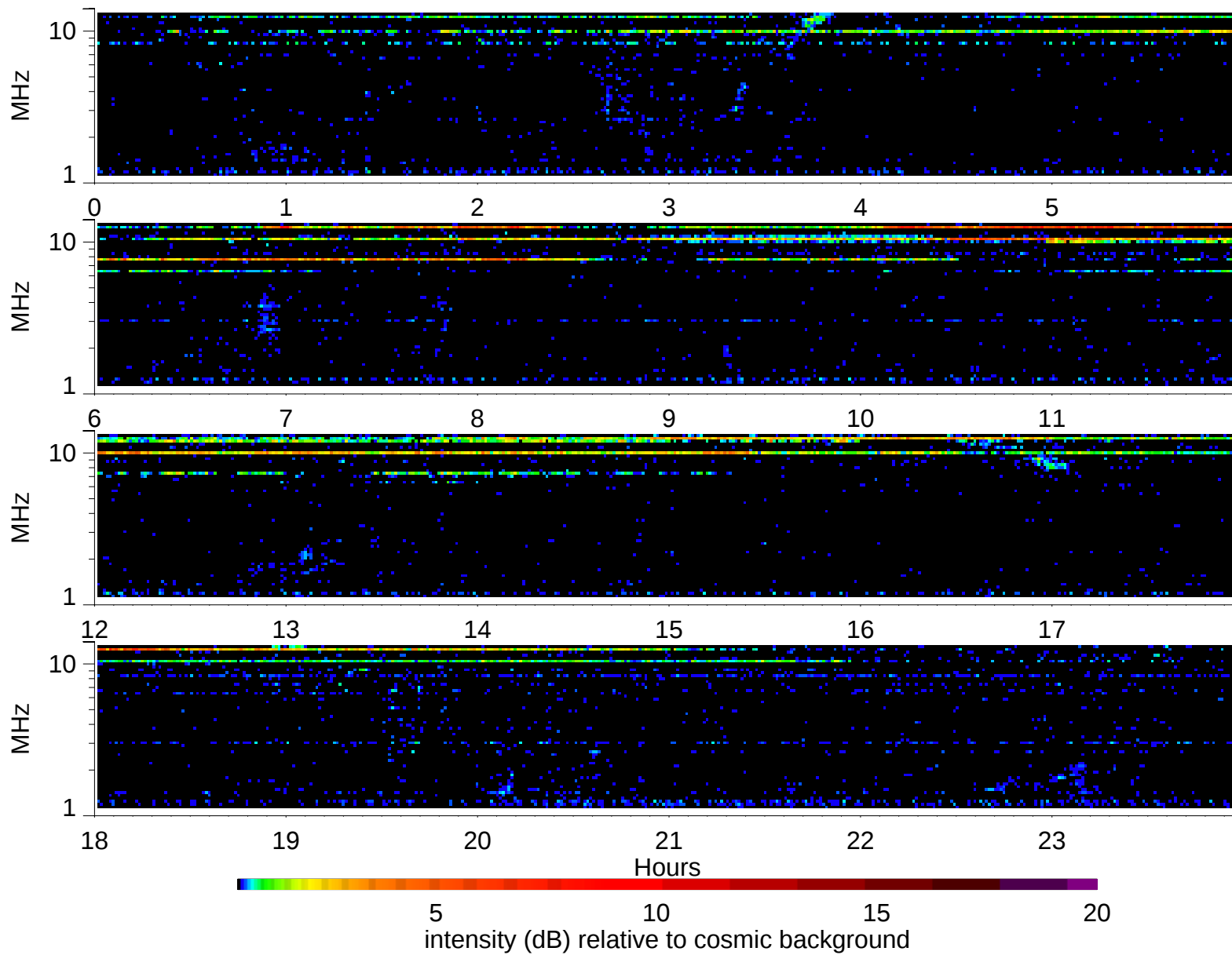
Wind Waves RAD2 receiver: 2006/6/4
