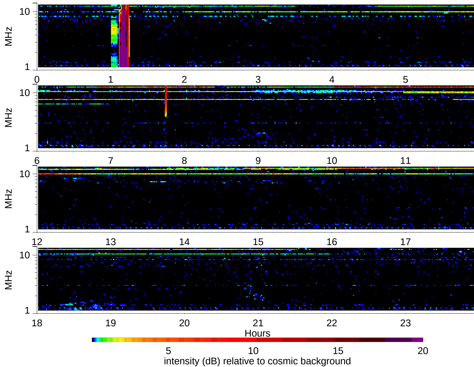
Wind Waves RAD2 receiver: 2006/6/5
