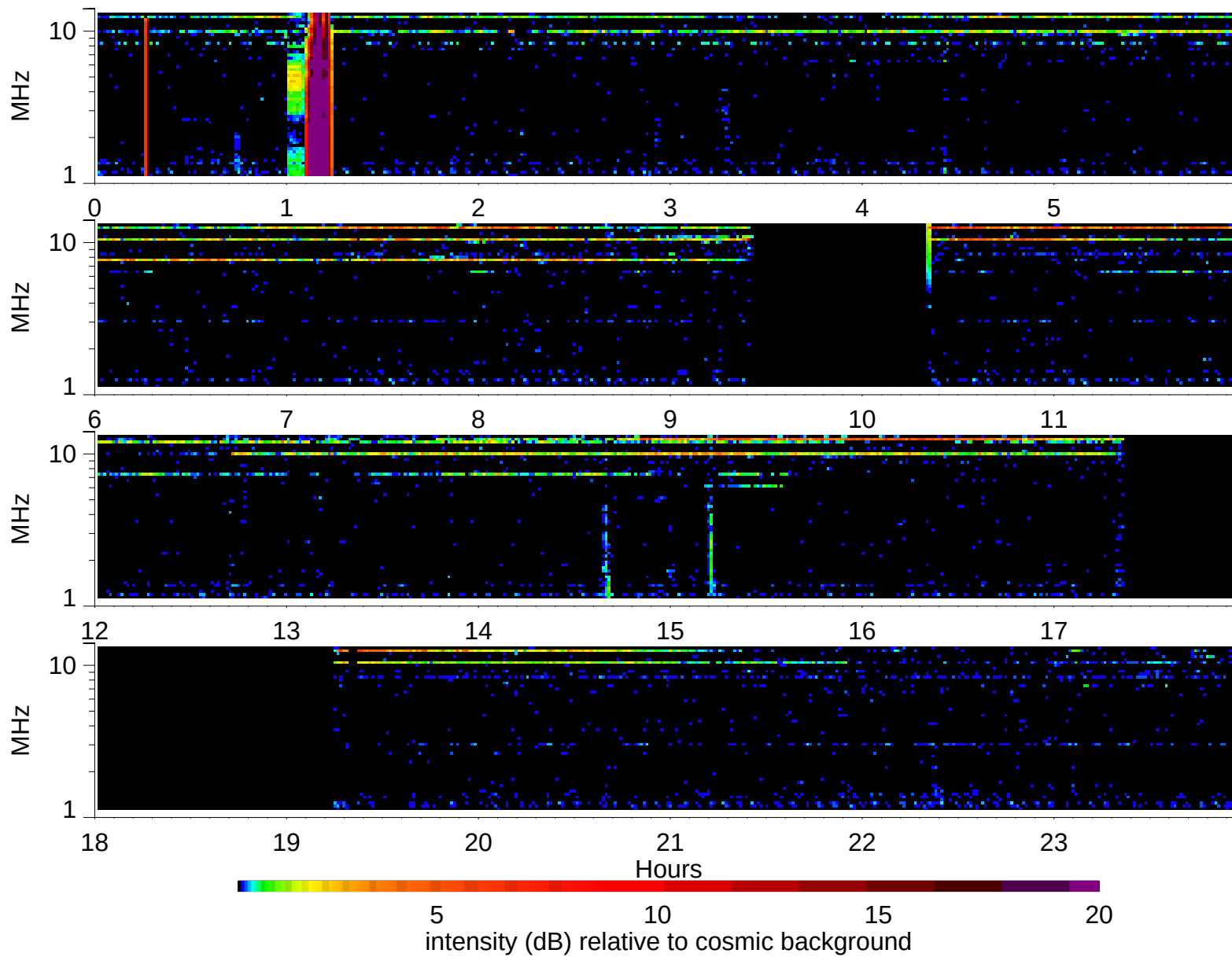
Wind Waves RAD2 receiver: 2006/6/9
