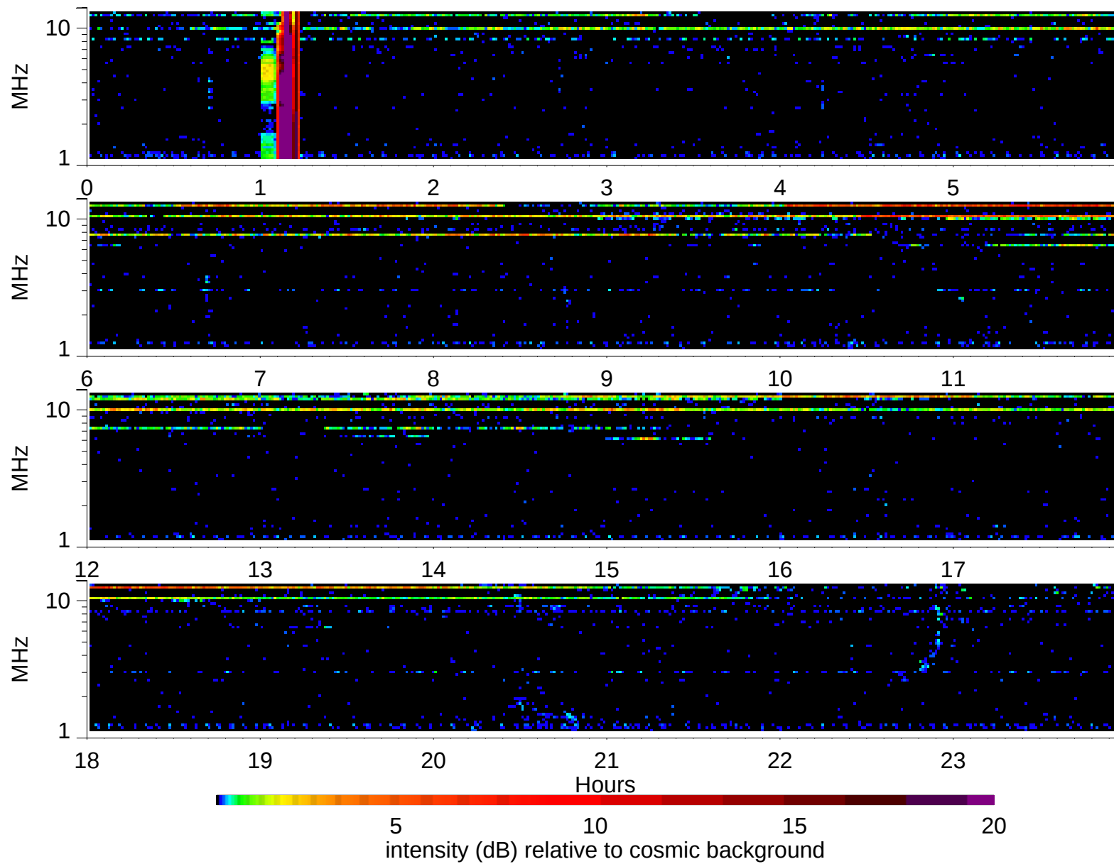
Wind Waves RAD2 receiver: 2006/6/11
