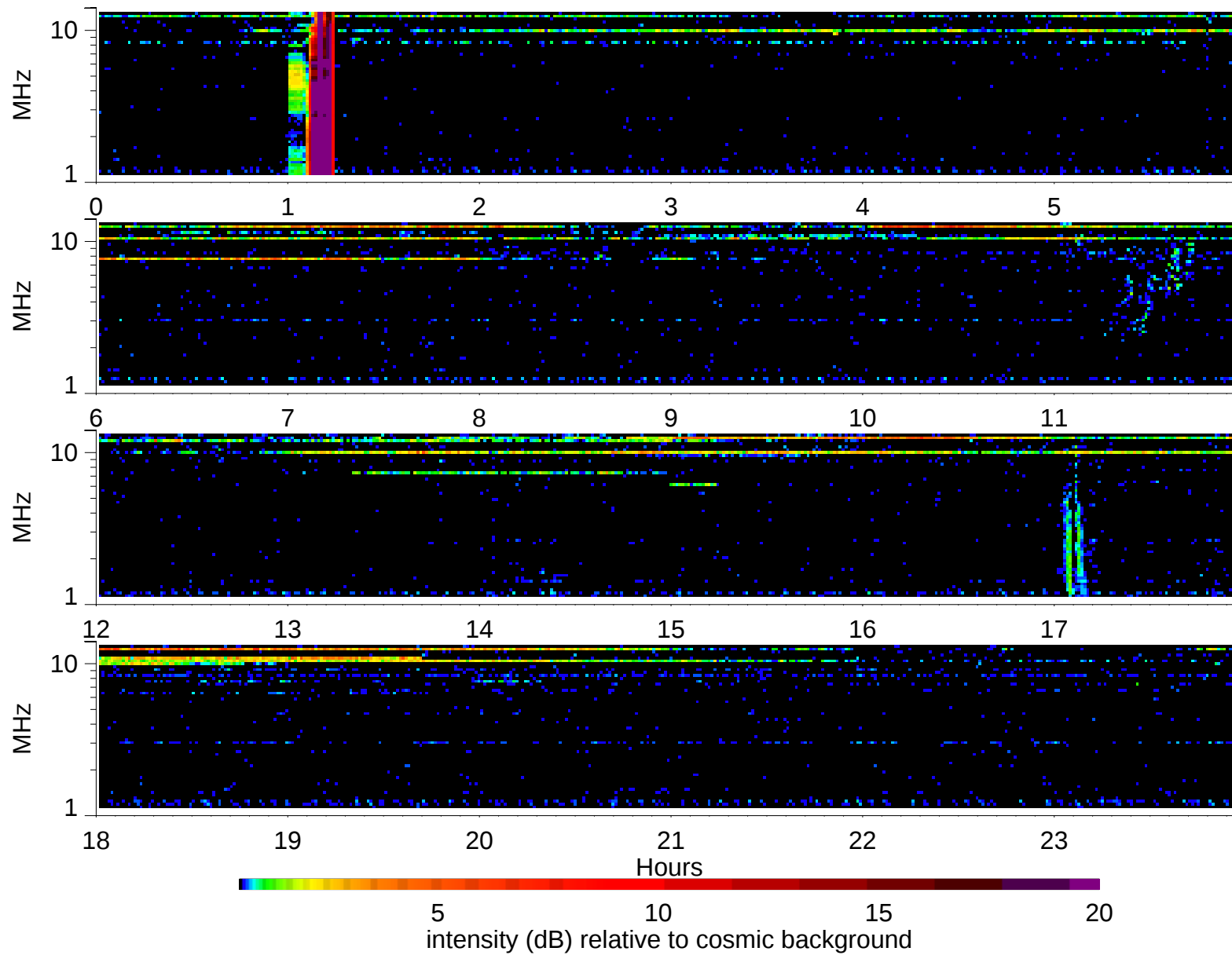
Wind Waves RAD2 receiver: 2006/6/15
