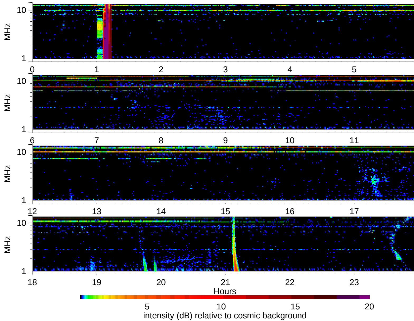
Wind Waves RAD2 receiver: 2006/6/19
