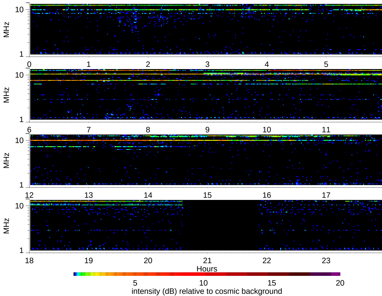
Wind Waves RAD2 receiver: 2006/6/26
