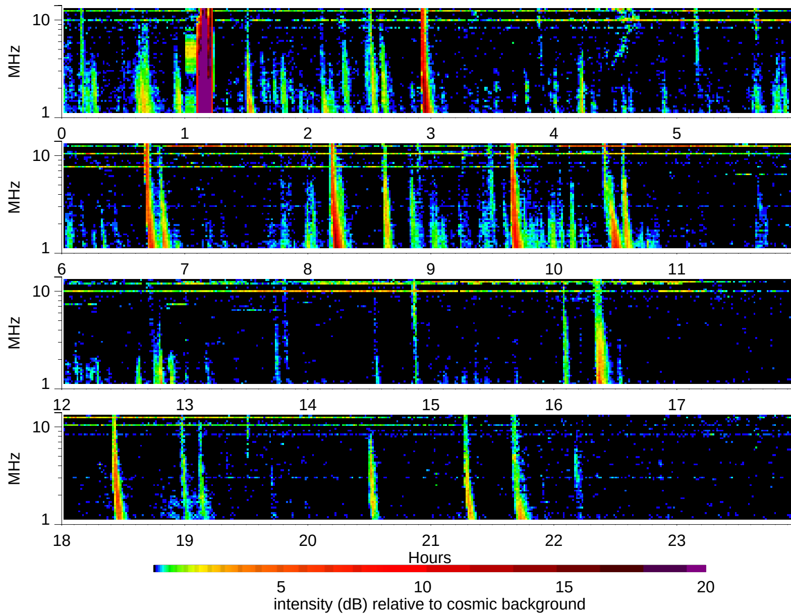
Wind Waves RAD2 receiver: 2006/7/3
