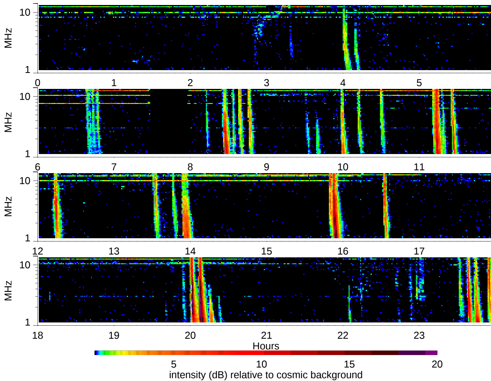
Wind Waves RAD2 receiver: 2006/7/4
