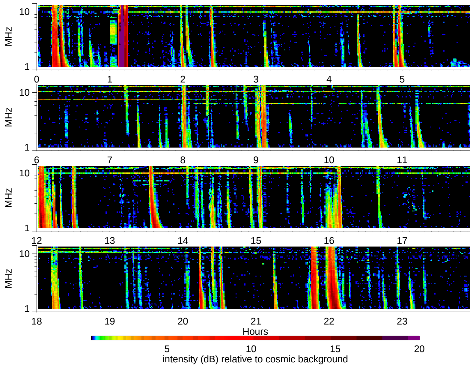
Wind Waves RAD2 receiver: 2006/7/7
