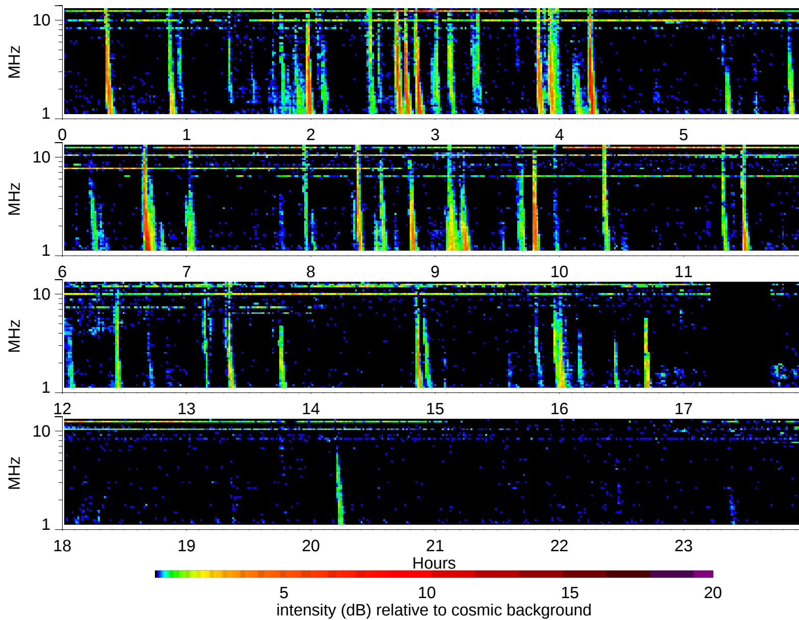
Wind Waves RAD2 receiver: 2006/7/8
