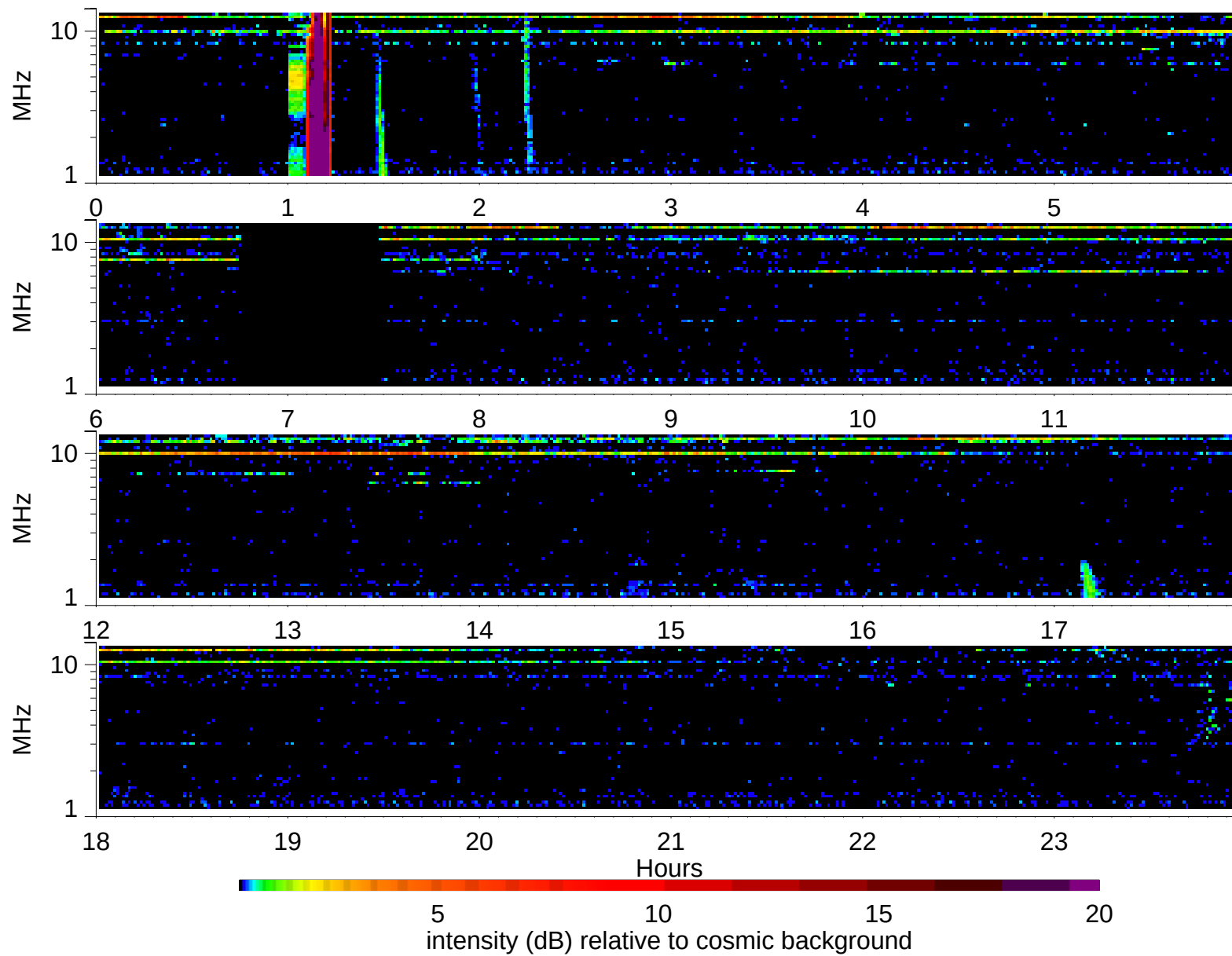
Wind Waves RAD2 receiver: 2006/7/11
