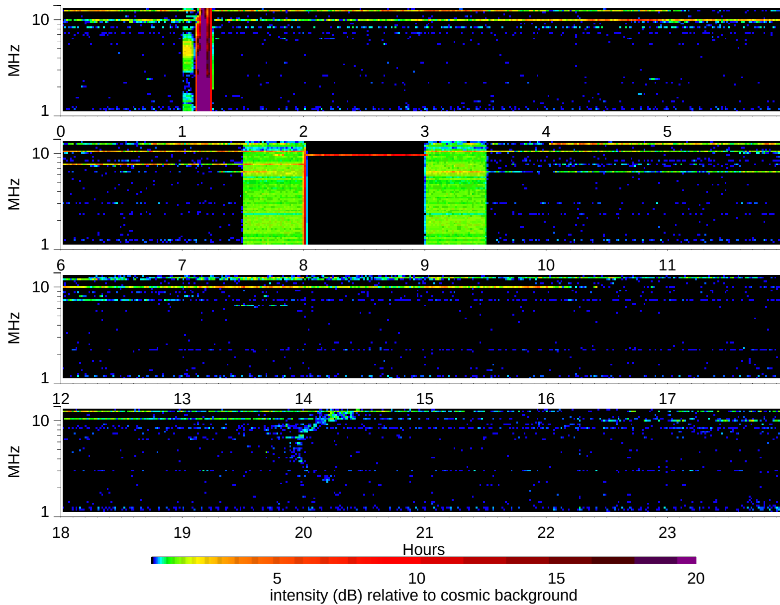
Wind Waves RAD2 receiver: 2006/7/21
