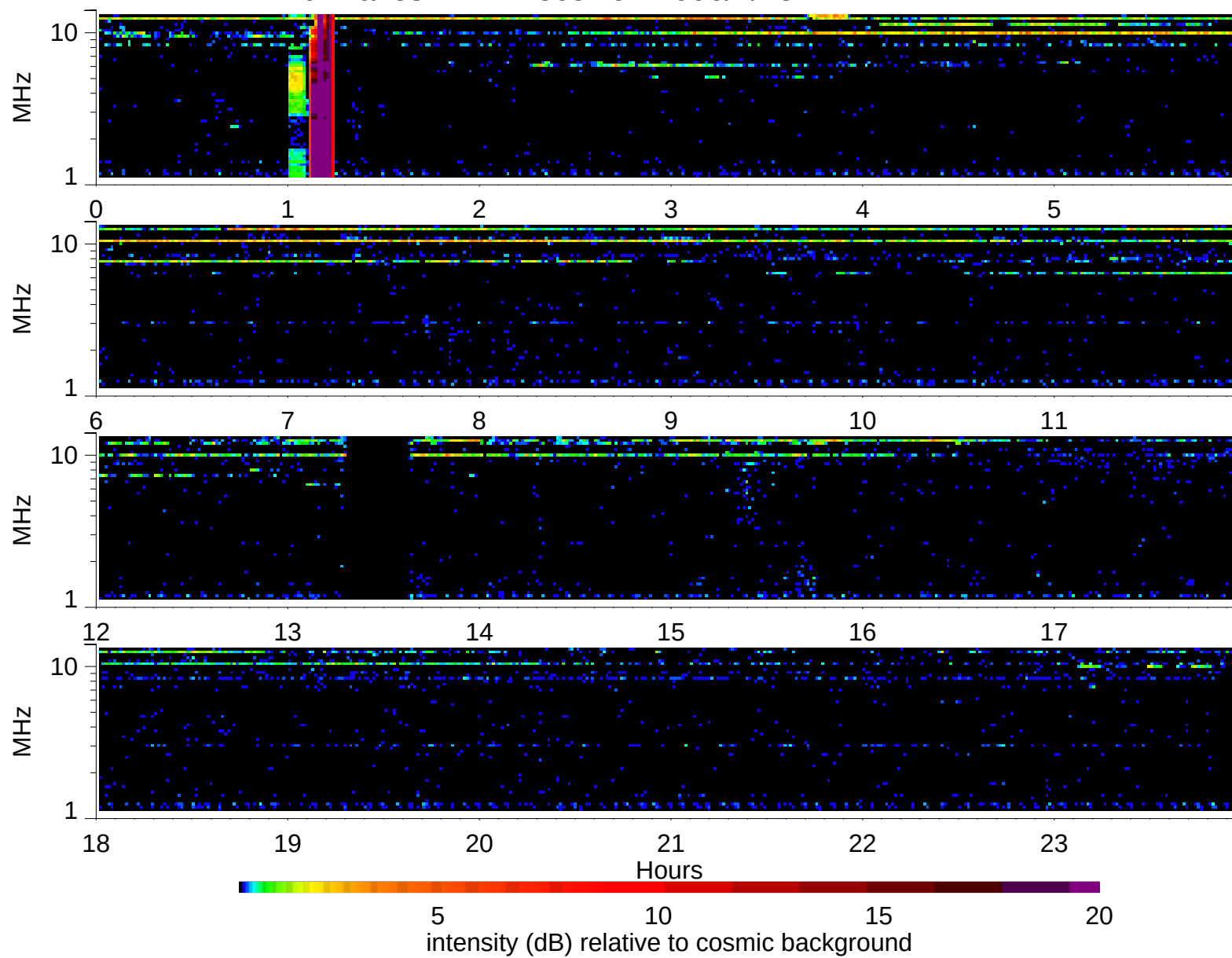
Wind Waves RAD2 receiver: 2006/7/23
