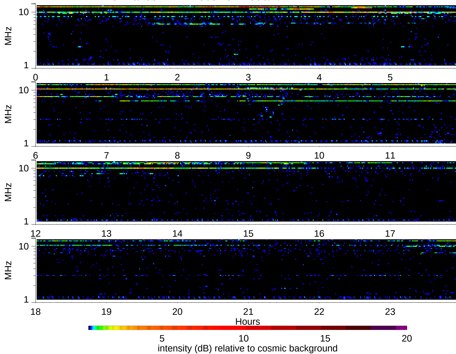
Wind Waves RAD2 receiver: 2006/7/24
