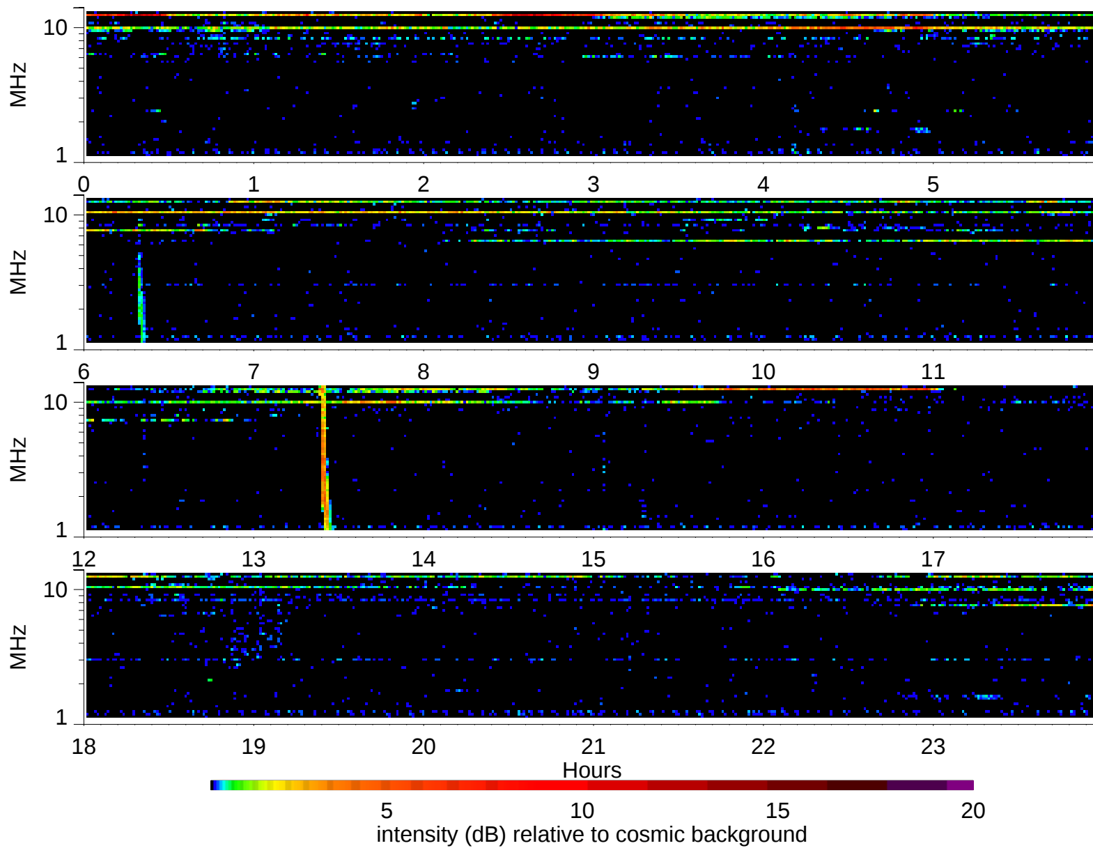
Wind Waves RAD2 receiver: 2006/8/5
