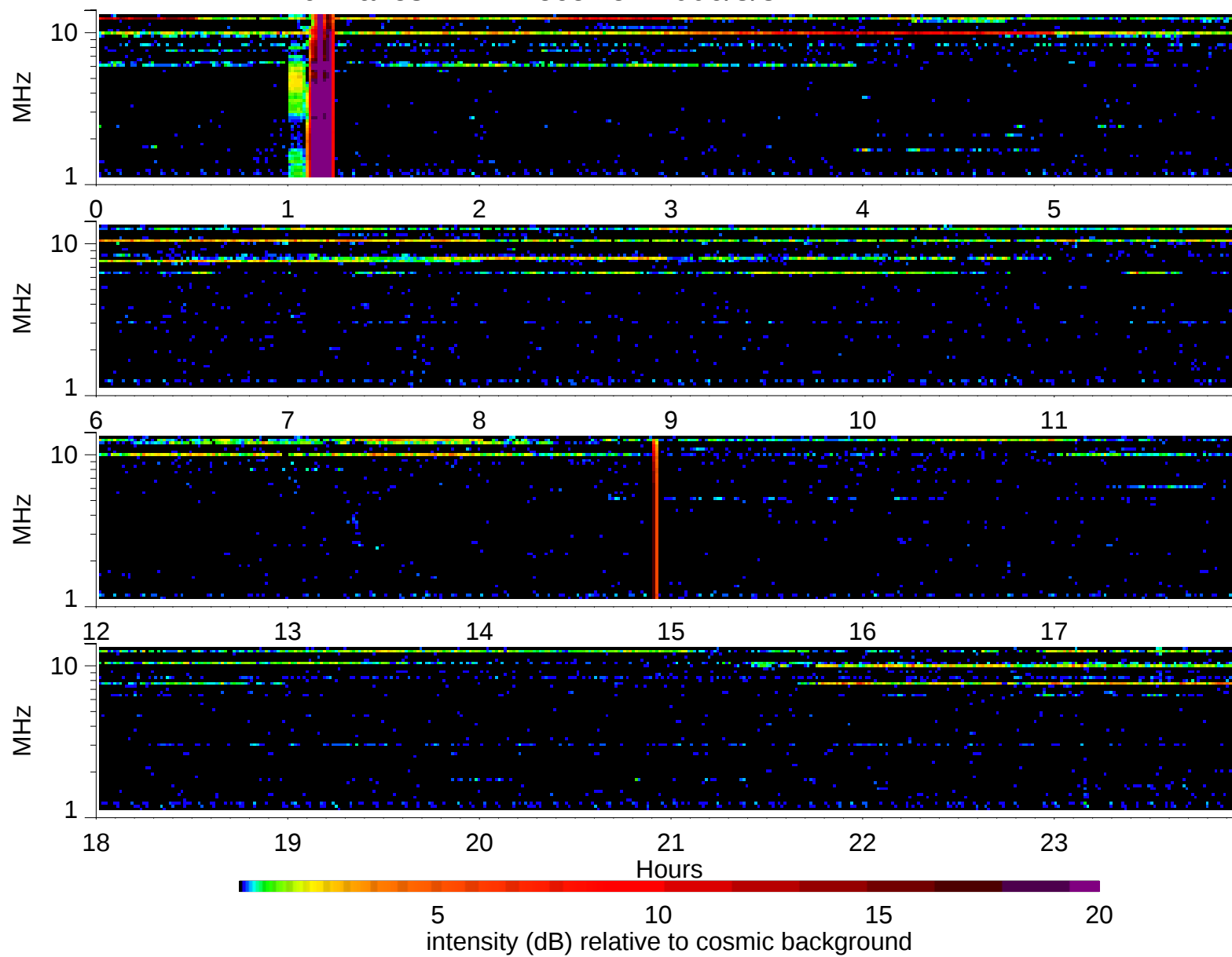
Wind Waves RAD2 receiver: 2006/8/8
