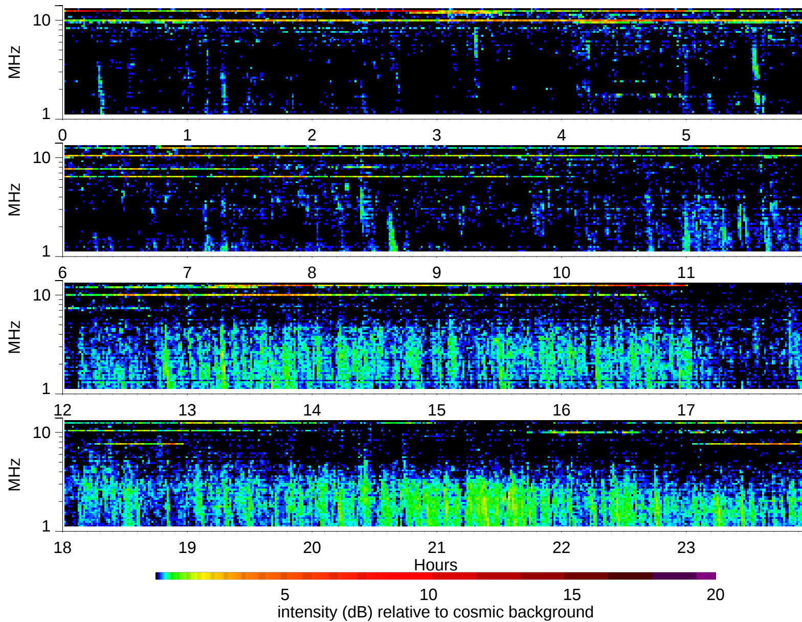
Wind Waves RAD2 receiver: 2006/8/13
