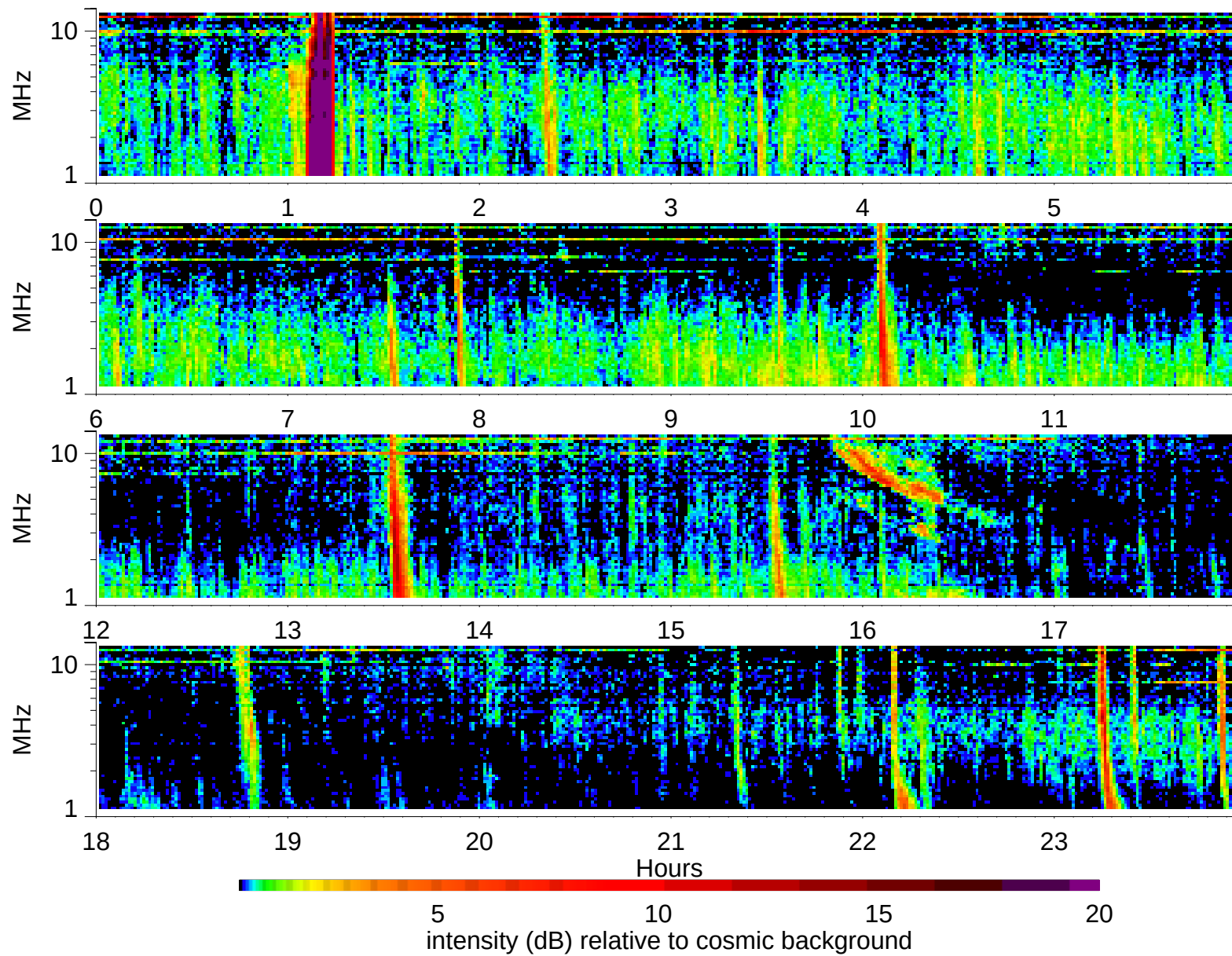
Wind Waves RAD2 receiver: 2006/8/16
