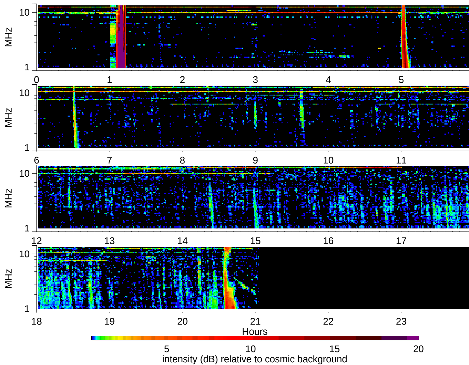
Wind Waves RAD2 receiver: 2006/8/26
