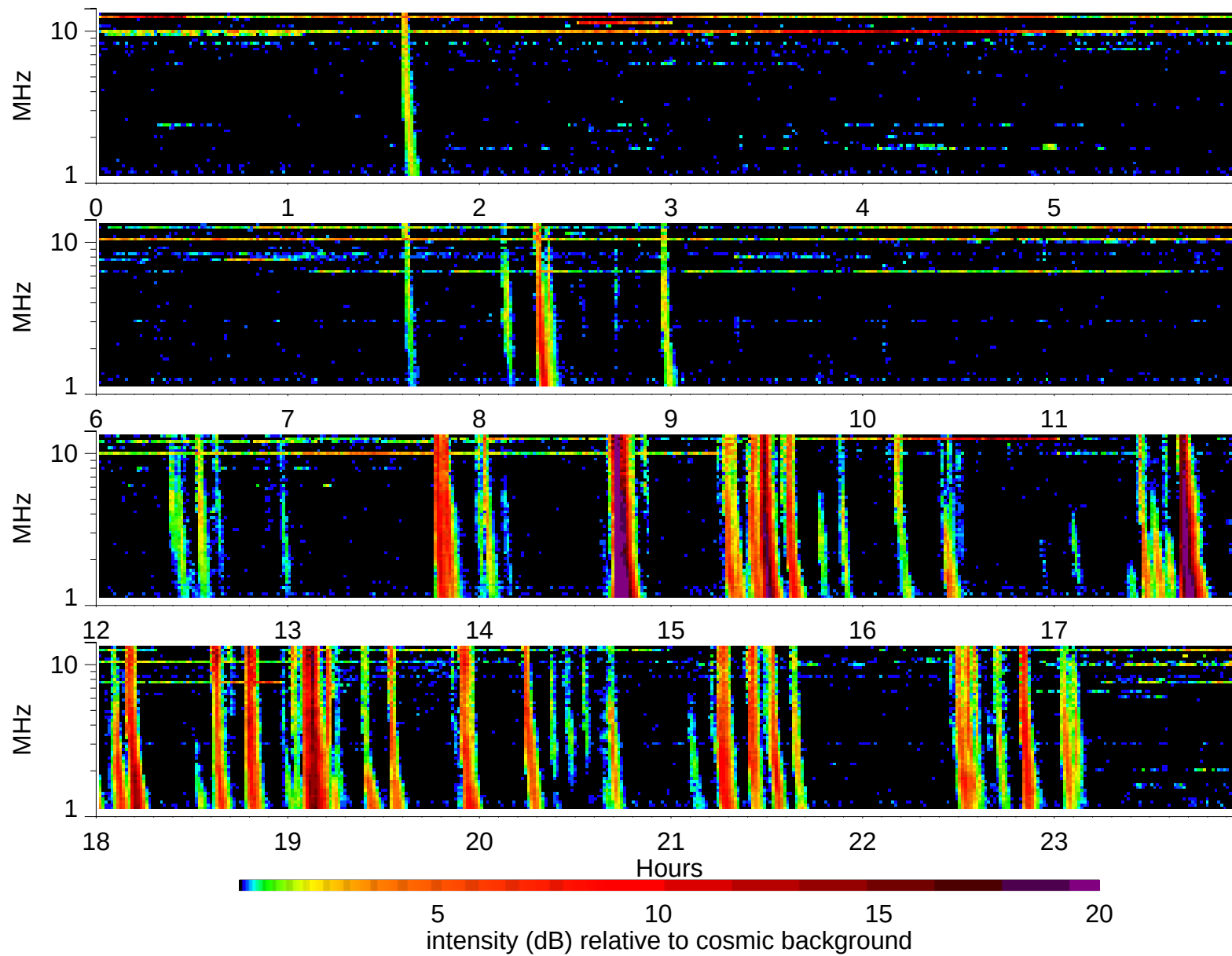
Wind Waves RAD2 receiver: 2006/8/29
