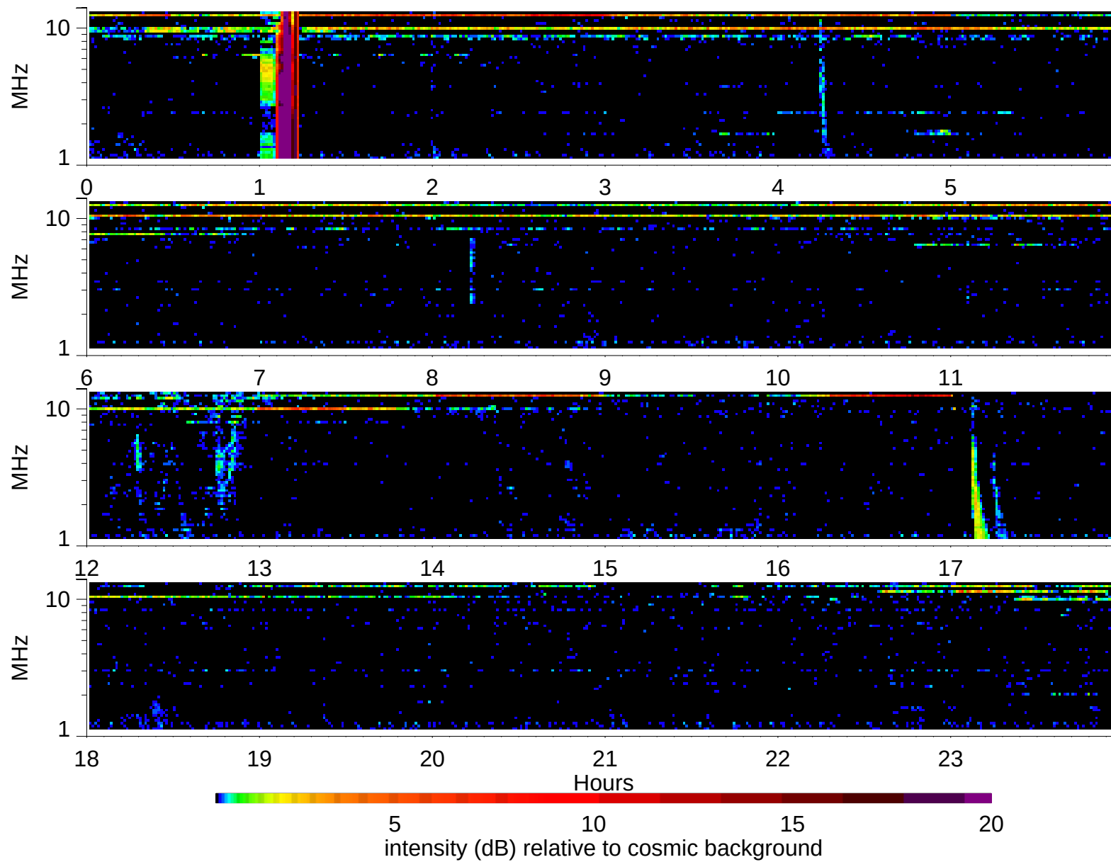
Wind Waves RAD2 receiver: 2006/9/3
