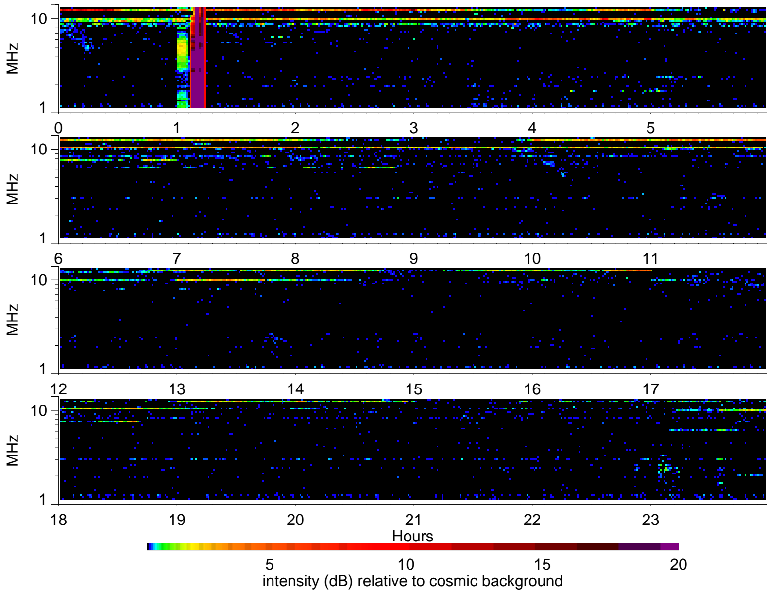
Wind Waves RAD2 receiver: 2006/9/7
