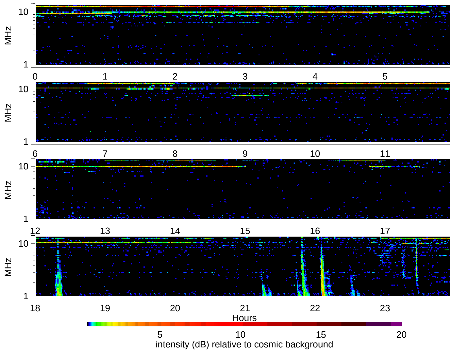
Wind Waves RAD2 receiver: 2006/9/12
