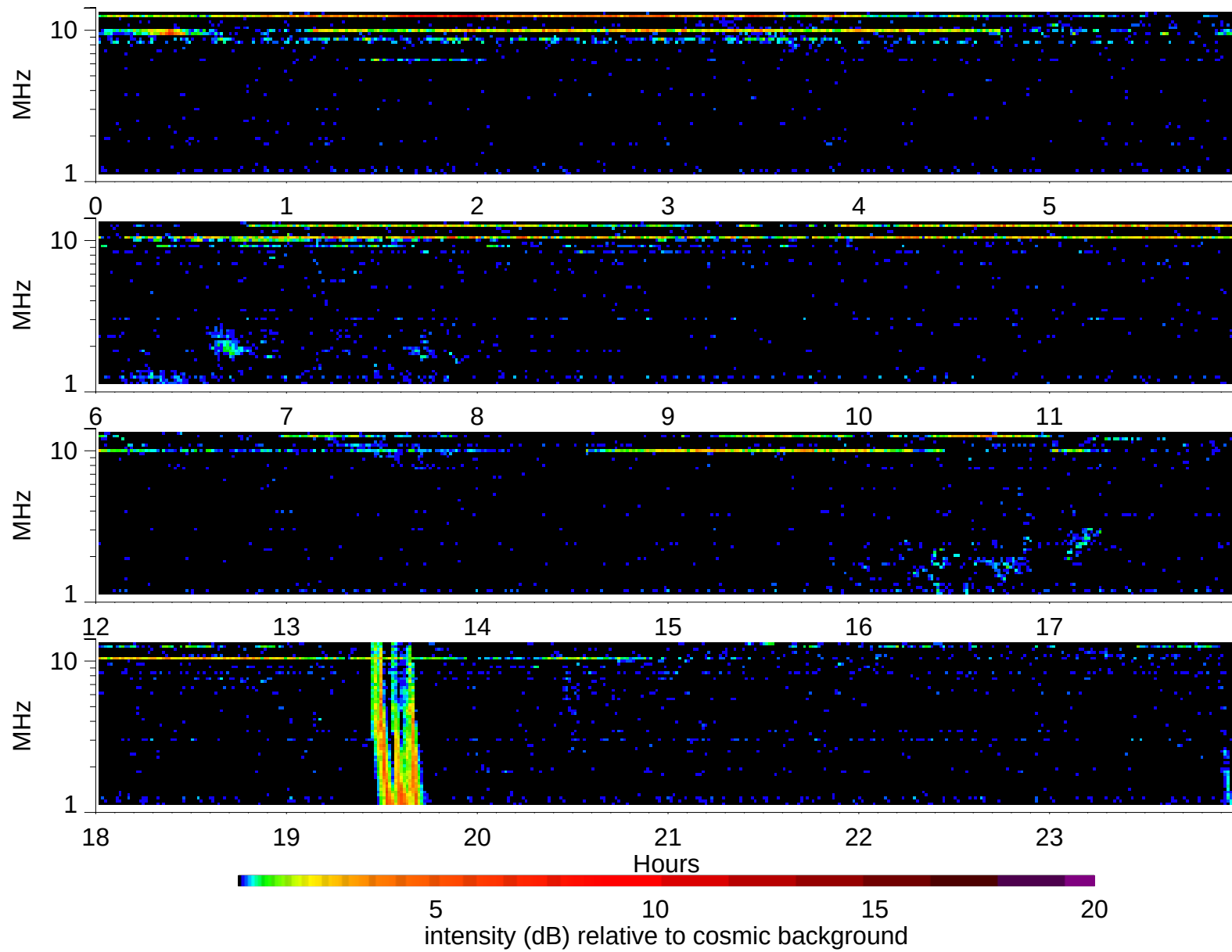
Wind Waves RAD2 receiver: 2006/9/18
