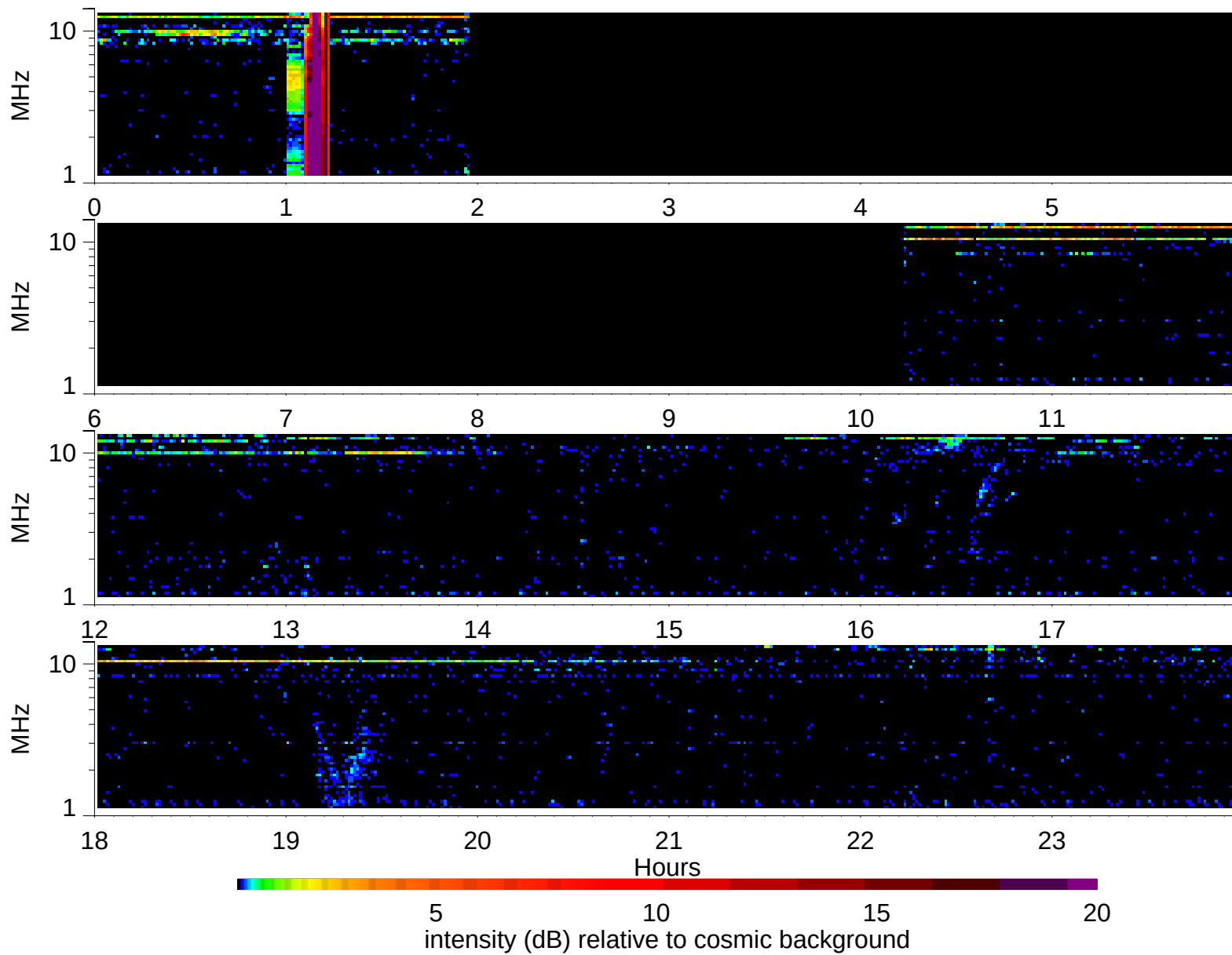
Wind Waves RAD2 receiver: 2006/9/19
