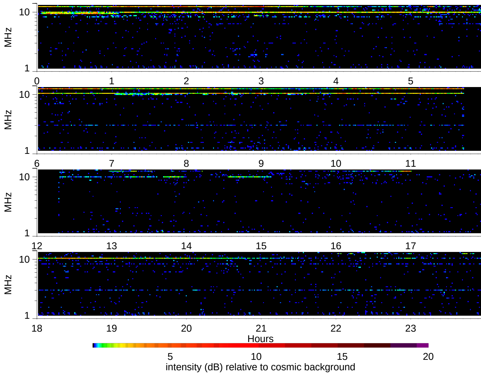
Wind Waves RAD2 receiver: 2006/9/20
