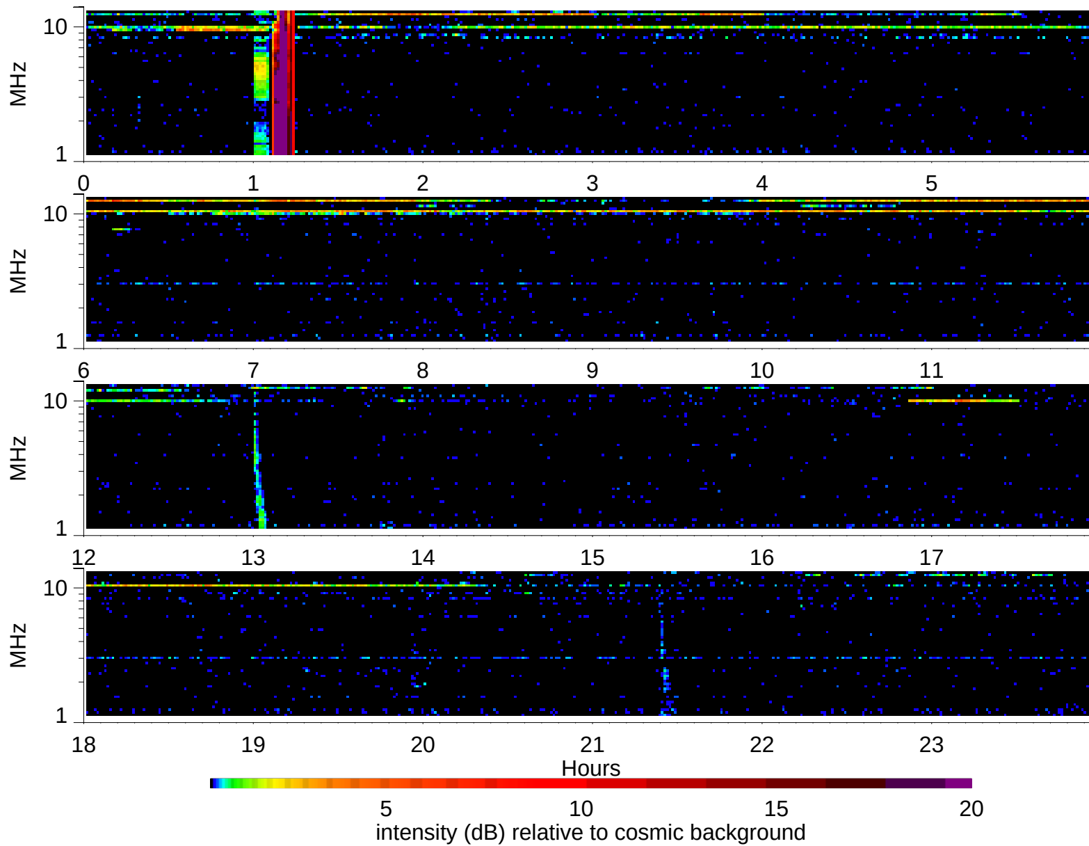
Wind Waves RAD2 receiver: 2006/9/21
