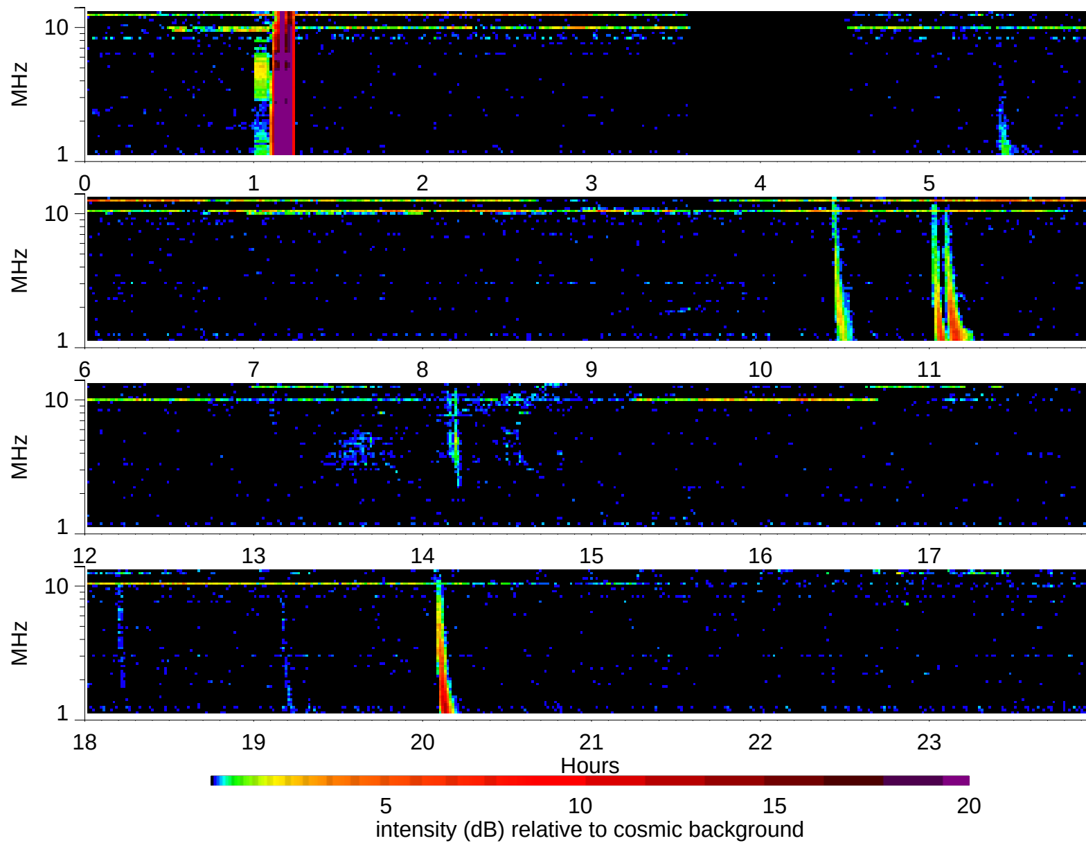
Wind Waves RAD2 receiver: 2006/9/23
