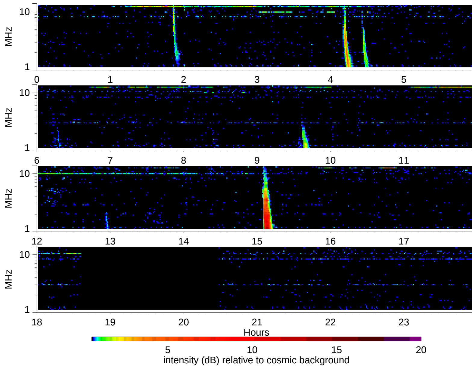
Wind Waves RAD2 receiver: 2006/10/8
