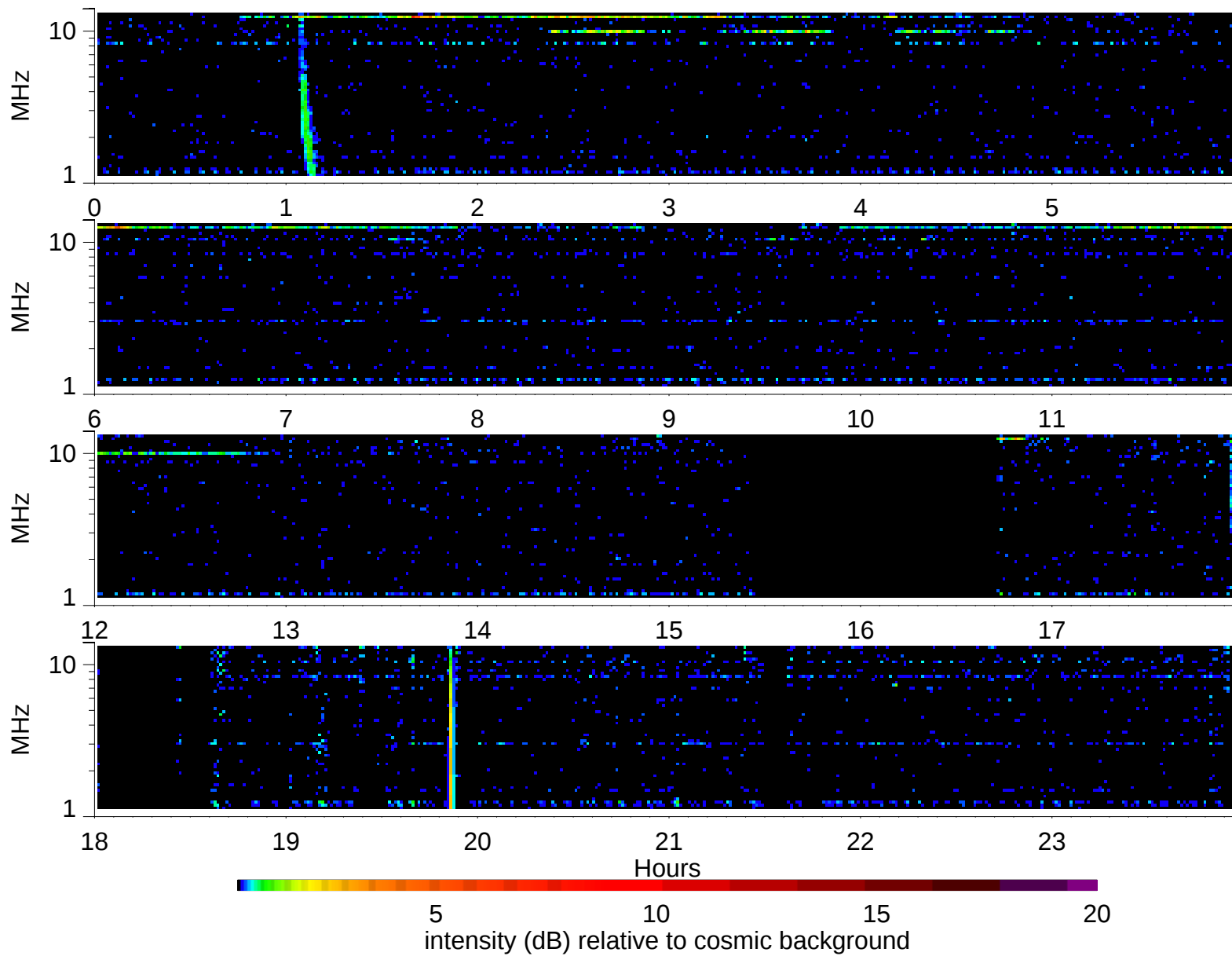
Wind Waves RAD2 receiver: 2006/10/10
