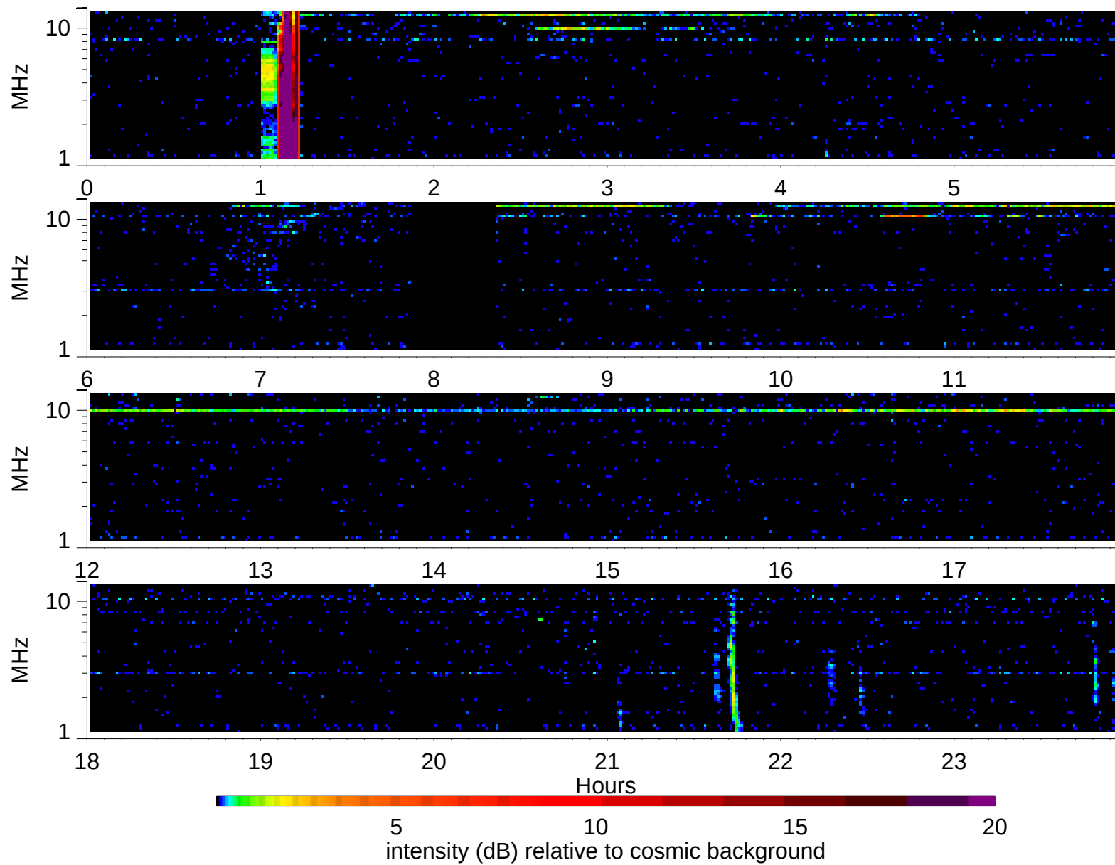
Wind Waves RAD2 receiver: 2006/10/11
