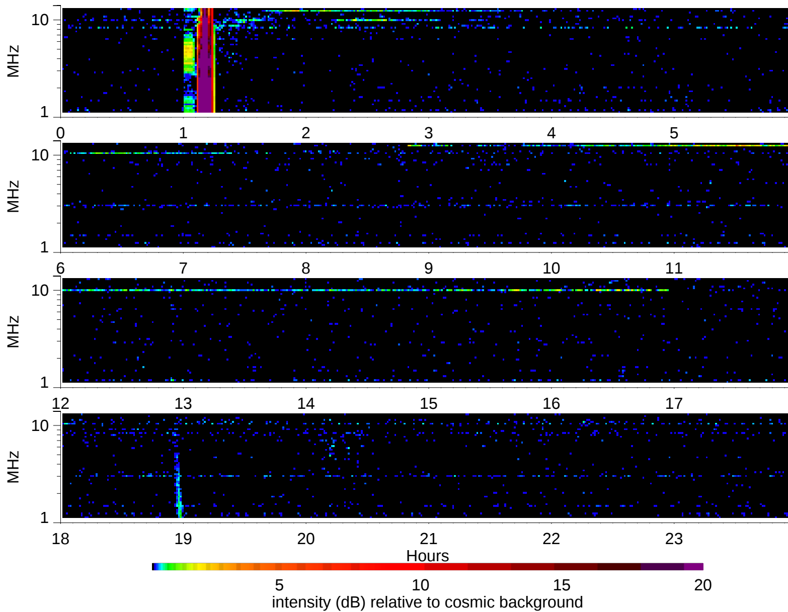
Wind Waves RAD2 receiver: 2006/10/13
