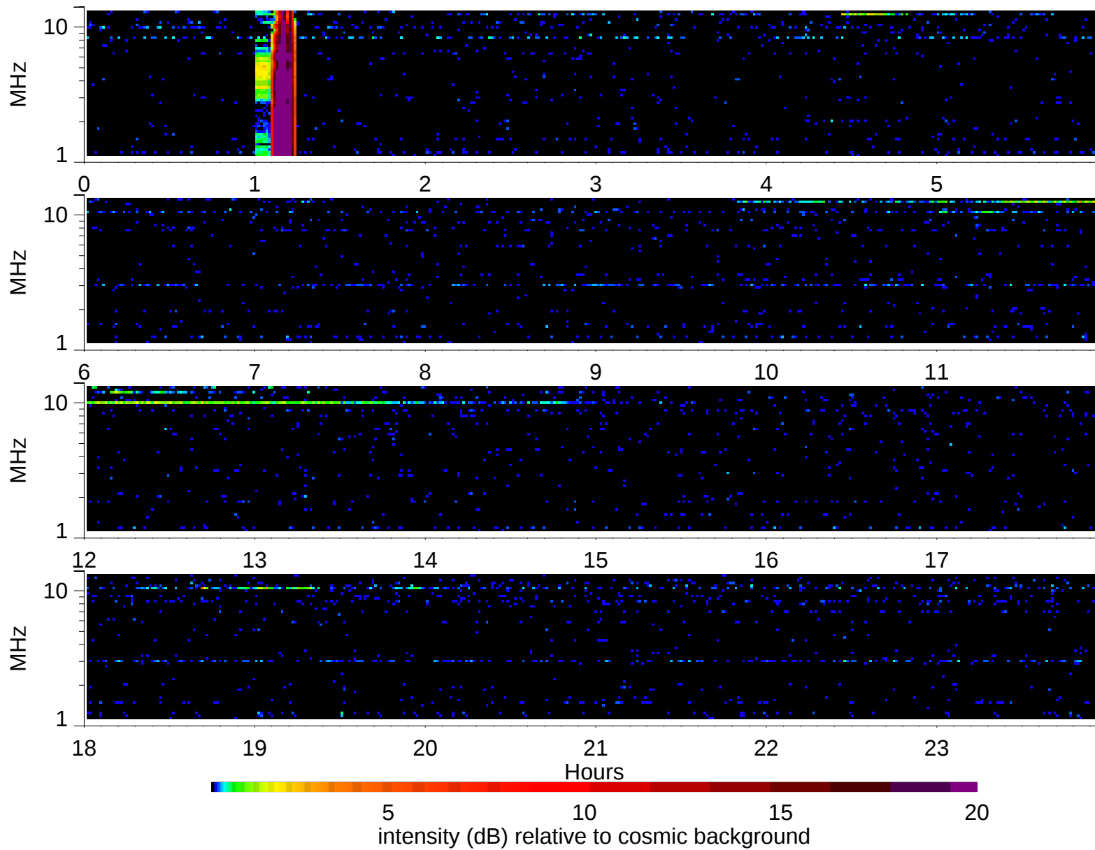
Wind Waves RAD2 receiver: 2006/10/17
