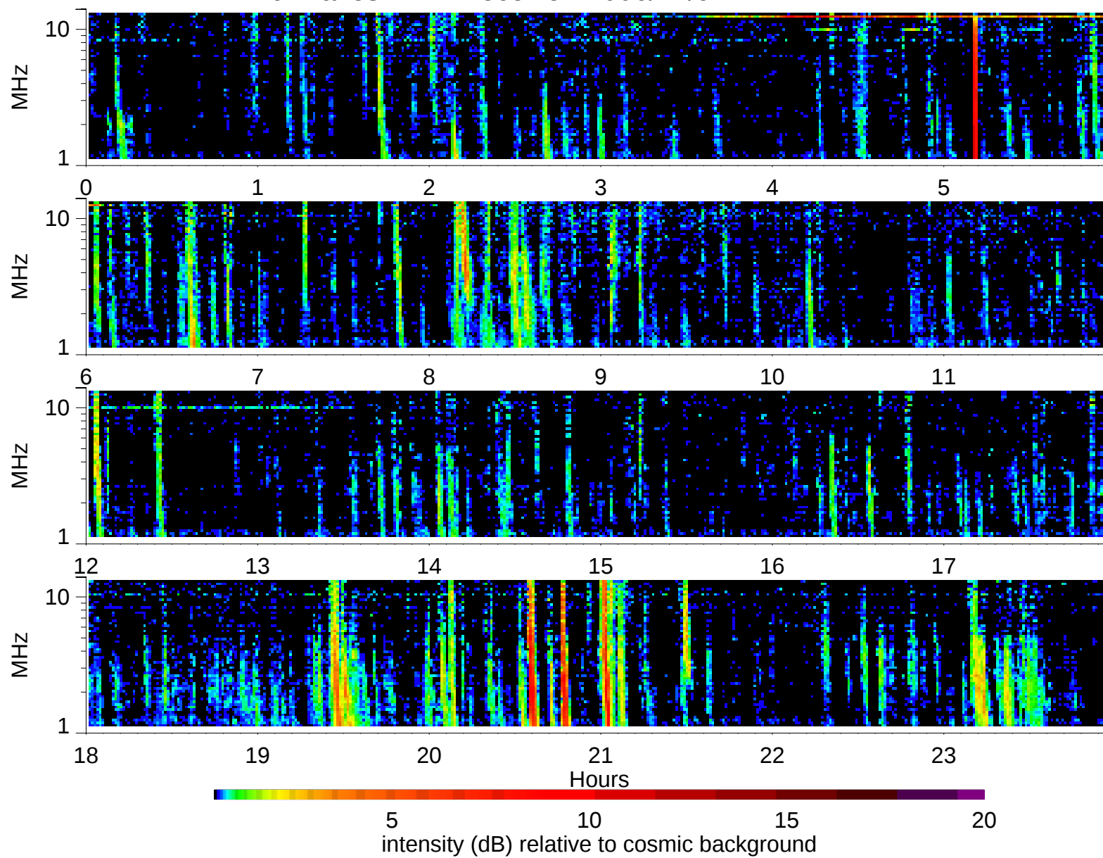
Wind Waves RAD2 receiver: 2006/11/9
