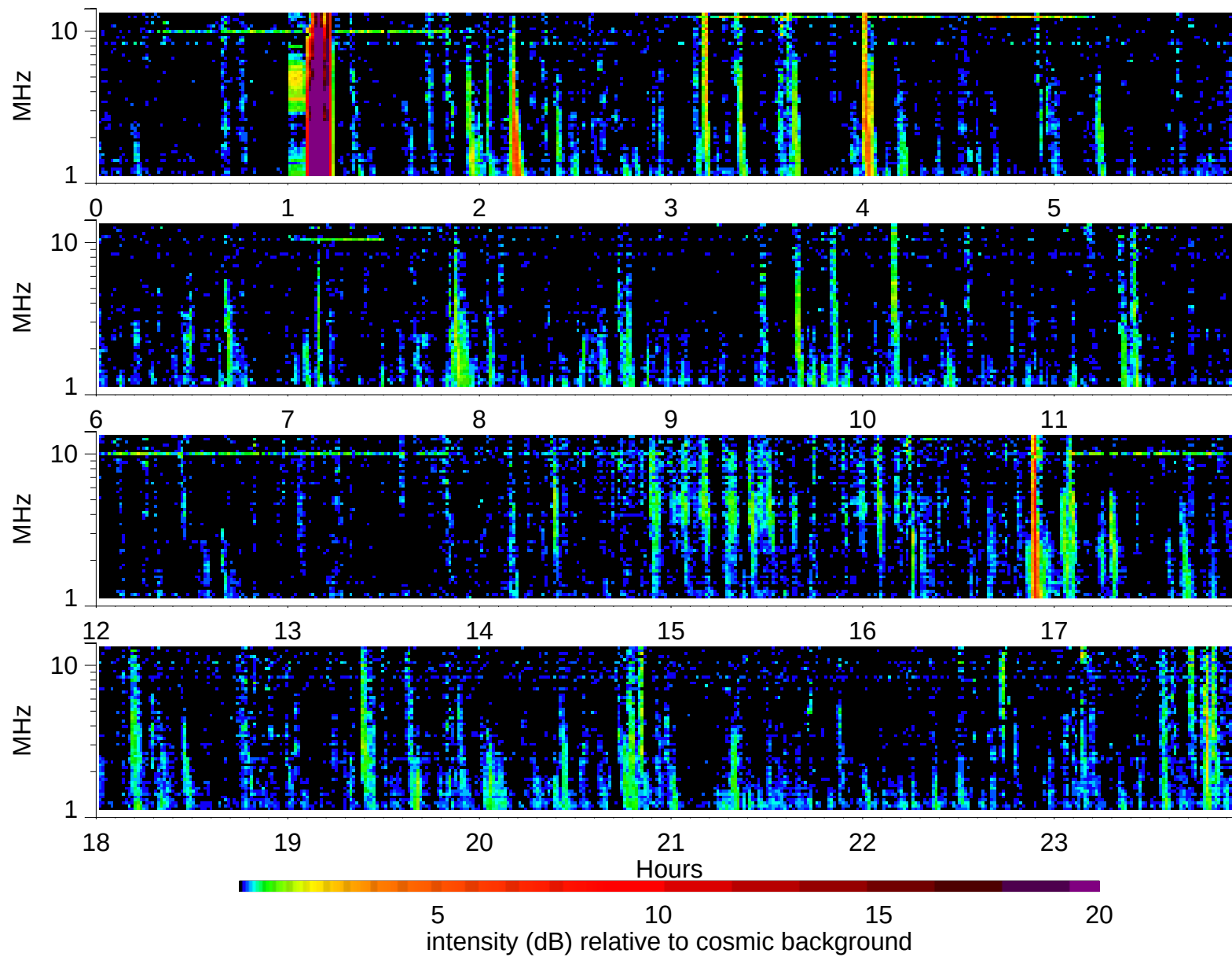
Wind Waves RAD2 receiver: 2006/11/10
