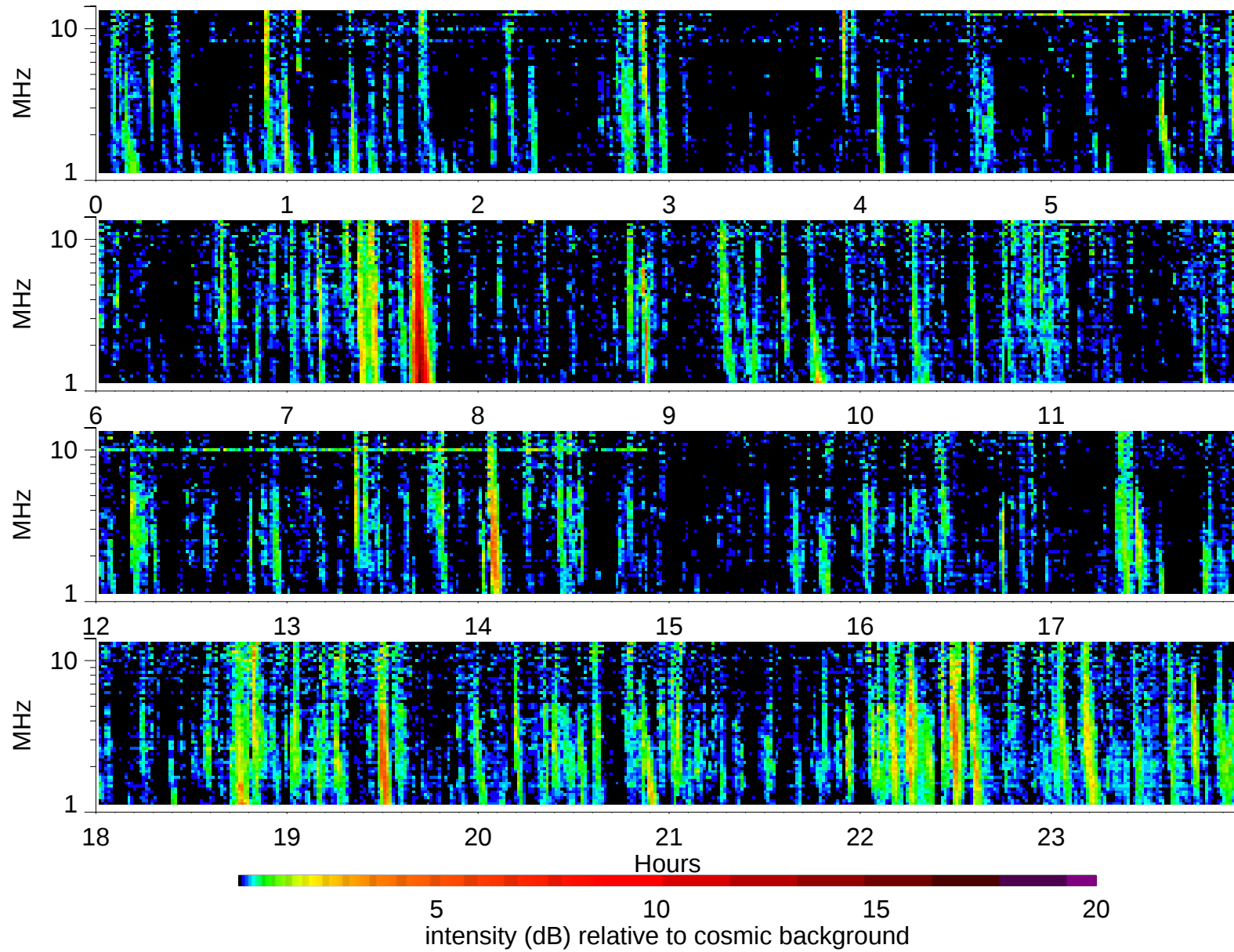
Wind Waves RAD2 receiver: 2006/11/11
