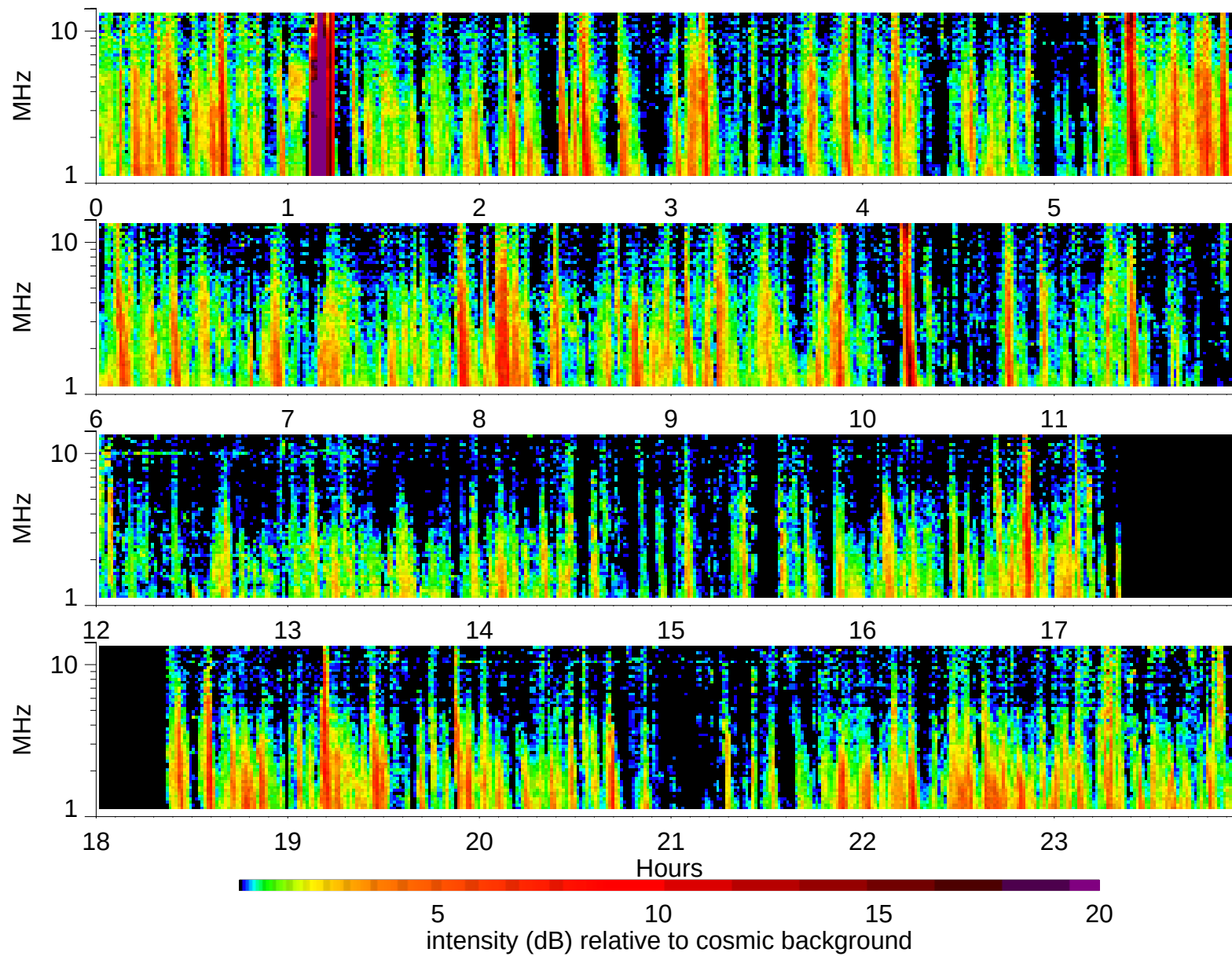
Wind Waves RAD2 receiver: 2006/11/14
