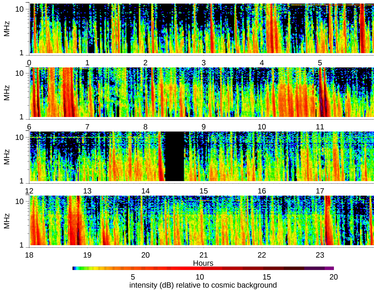
Wind Waves RAD2 receiver: 2006/11/15
