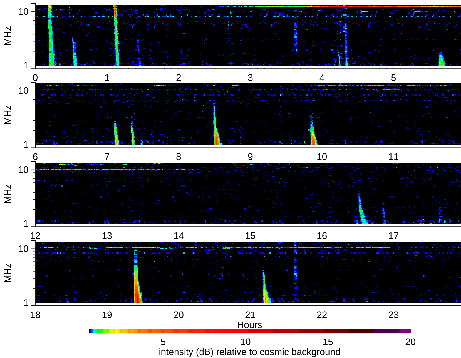
Wind Waves RAD2 receiver: 2006/11/21
